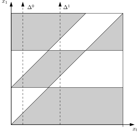
Figure 4: The partition of \mathbb{R}^2 defined by the pieces of Q . In this example, there are two value functions in B_i : A reward function R_1(x_1) at the origin of the horizontal faces in the figure, and a function R_{01}(x_1 - x_0) that represents piecewise linear preferences on the difference between x_0 and x_1 and that induces the diagonal constraints. This is a standard situation encountered in many STPPs. The axis \Delta^0 and \Delta^1 traverse the same sequence of pieces of both R_1 and R_{01} . However, they traverse different pieces of Q .
