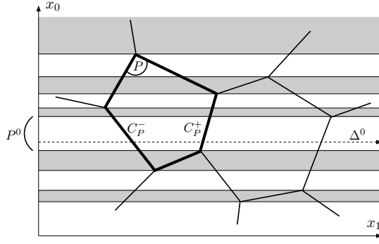
Figure 2: Projecting of Q on X_{-i} = \{x_0\} : The convex polygonal partition of the plane represents the pieces of Q . Horizontal stripes represents the partition of \mathbb{R}[X_{-i}] obtained by projecting Q .
