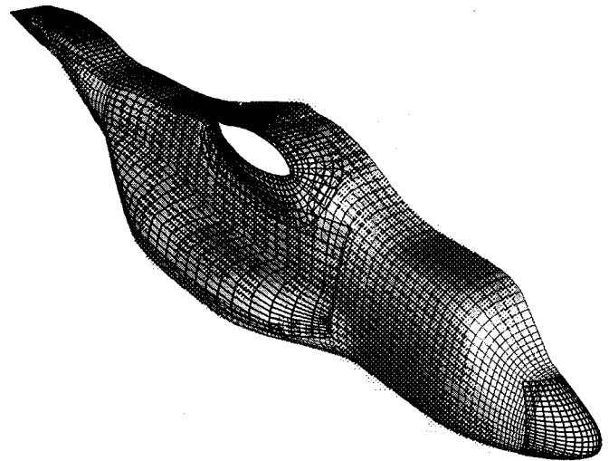
Figure 8. Overlapping seam and block surface grids for the V-22 tiltrotor fuselage (seam grids are drawn with thicker and darker lines).
