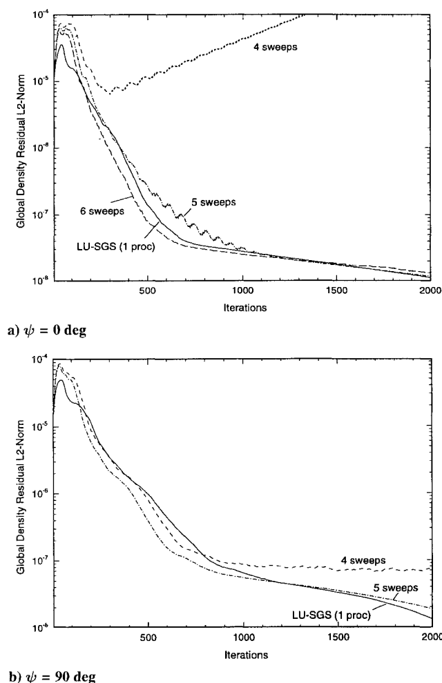
Fig. 3 Convergence with DP-LUR operator.
