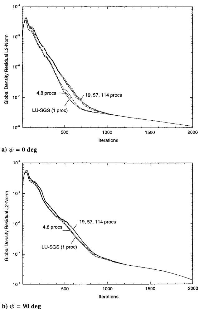
Fig. 4 Convergence with hybrid operator ( i_{\text{sweep}} = 1 ).
