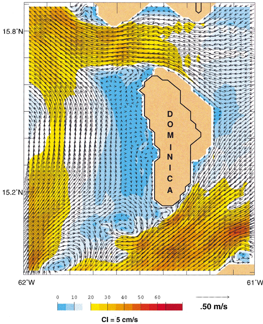
Fig. 5. Snapshot of layer one current vectors (arrows) superimposed on current speed (color) for a 1^\circ square surrounding the island of Dominica in the Lesser Antilles island chain from 1/64^\circ , five-layer simulation 64H in Table 1. The location is marked as a red box on Fig. 4d for reference. Every current vector on the 1/64^\circ grid is plotted. The contour interval of the current speed is 5 \text{ cm s}^{-1} .
