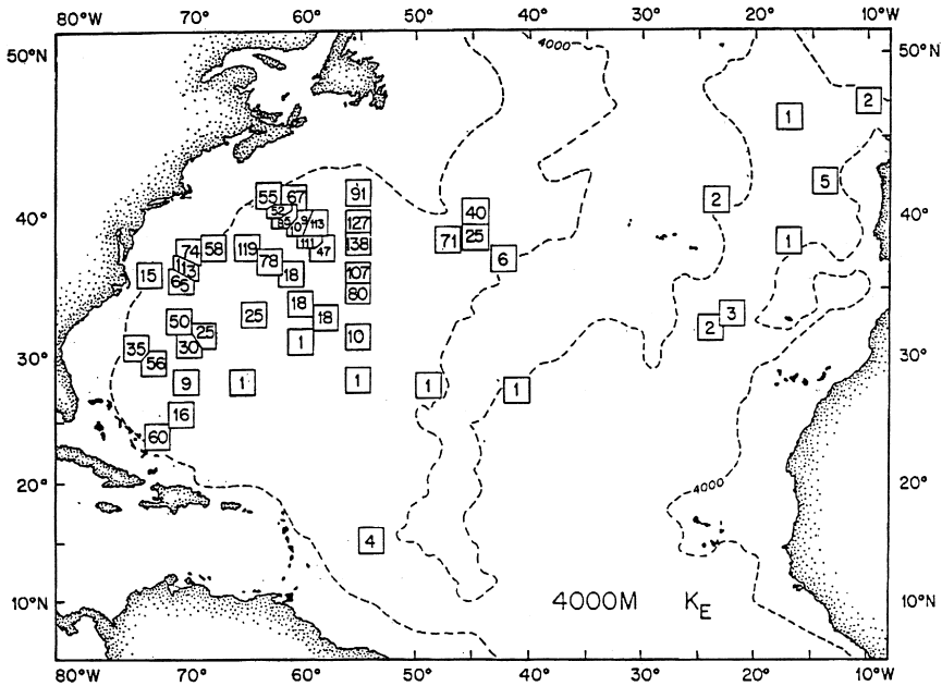
Fig. 13. . Abyssal ( \sim 4000 m depth) EKE ( \text{cm}^2 \text{s}^{-2} ) in the Atlantic Ocean determined from current meter data (from Schmitz, 1984, 1996).
