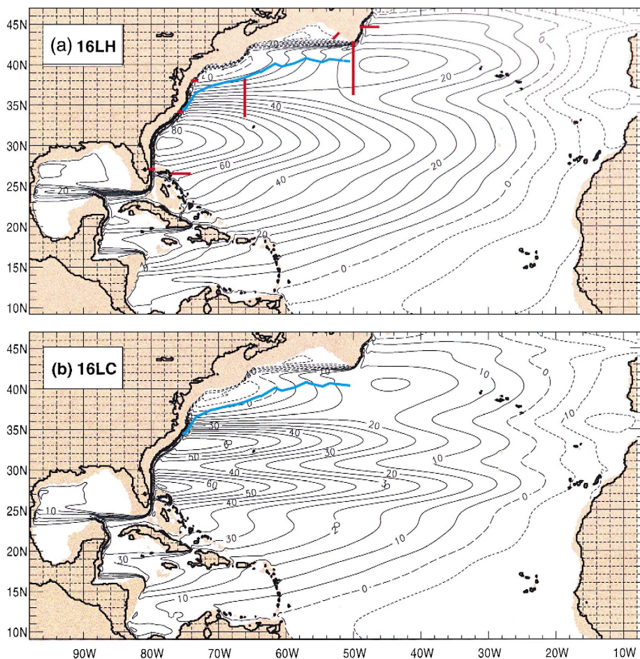
Fig. 2. Whole domain mean sea surface height (SSH) from two 1/16^\circ , 1.5-layer linear reduced-gravity simulations. (a) Simulation 16LH (Table 1) forced by the Hellerman and Rosenstein (1983) monthly wind stress climatology, and (b) simulation 16LC forced by the COADS (da Silva et al., 1994a,b) monthly wind stress climatology. The mean axis of the Gulf Stream from TOPEX/Poseidon altimetry (Lee et al., 1997) is superimposed. The contour interval is 5 cm. Selected transport sections are marked on (a). The section marked for the Gulf Stream at 68^\circ\text{W} is the section used for linear simulation 16LH. The N–S limits of this section were adjusted for each simulation to capture the modeled Gulf Stream transport at 68^\circ\text{W} .
