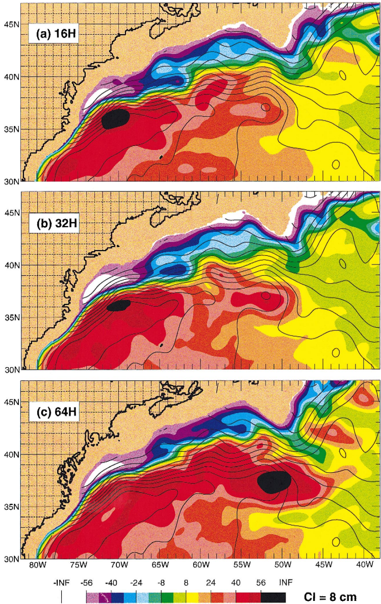
Fig. 8. Mean SSH (color) in the Gulf Stream region from (a) 1/16^\circ simulation 16H, (b) 1/32^\circ simulation 32H, and (c) 1/64^\circ simulation 64H. Superimposed on each are contours of surface dynamic height with respect to 1000 db from the Navy's GDEM oceanic climatology (Teague et al., 1990). Contour interval for the surface dynamic height and the model mean SSH is 8 cm.
