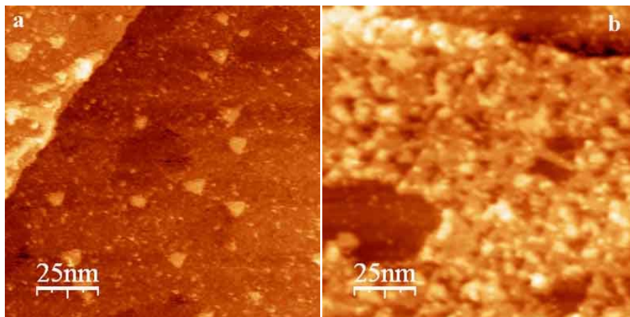
Figure 3. Large-scale EC-STM images of polyTEDOT-TTB on Au(111) acquired in 0.10 M HClO 4 at E = 0.20 V (vs RHE). The images were acquired after the Au(111) electrodes with TEDOT-TTB adlayer ((a) 2 μM and (b) 10 μM.) were scanned in the potential range of 0.2-1.2 V (vs RHE) in 0.10 M HClO 4 for 3 cycles. The bias voltage and the tunneling current were -22 mV and 100 pA, respectively.
