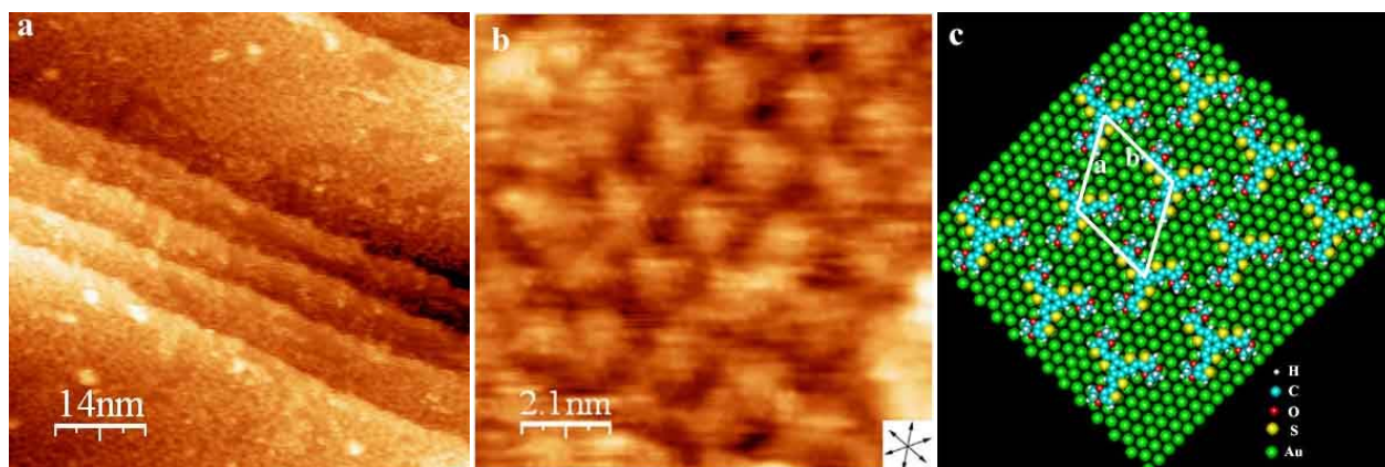
Figure 2 Large scale (a) and high-resolution (b) EC-STM images of TEDOT-TTB adlayer on Au(111) surface acquired in 0.10 M HClO 4 at E = 0.20 V (vs RHE). The bias voltage and the tunneling current were -22 mV and 100 pA, respectively. The set of three arrows in Figure b indicated the close-packed directions. Proposed model and unit cell of TEDOT-TTB adlayer on the Au(111) surface (c).
