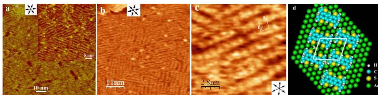
Figure 6. Large-scale (a, b) and high-resolution (c) STM images of 2TTA adlayer on Au(111) surface acquired in air (a) and in 0.10 M HClO 4 at E = 0.20 V (vs RHE) (b, c). The bias voltage and the tunneling current were 0.75 V and 200 pA for image (a) and 0.25 V and 100 pA for image (b, c), respectively. The set of three arrows indicated the close-packed directions.
