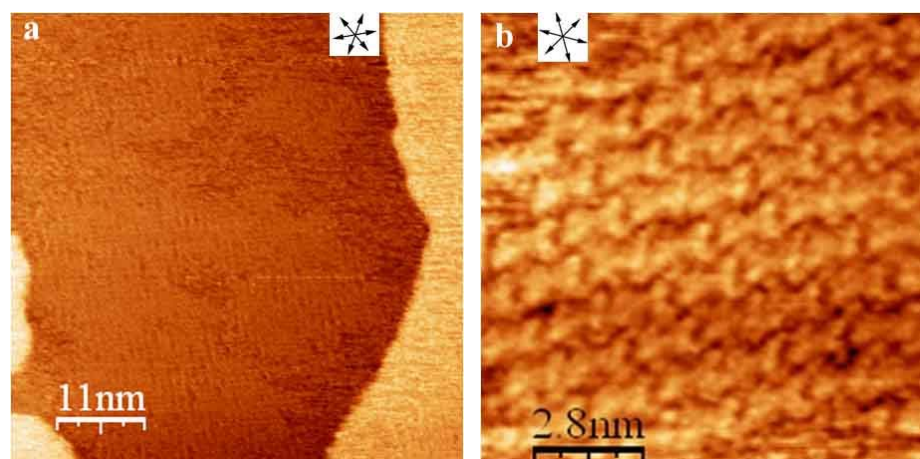
Figure 4. Large scale (a) and high-resolution (b) STM images of 3TTA adlayer on Au(111) acquired in 0.10 M HClO _4 at E = 0.60 V (vs RHE). The bias voltage and the tunneling current were 150 mV and 100 pA, respectively. The set of three arrows indicated the close-packed directions.
