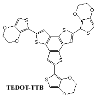
Chart 1. Chemical structure of TEDOT-TTB.
