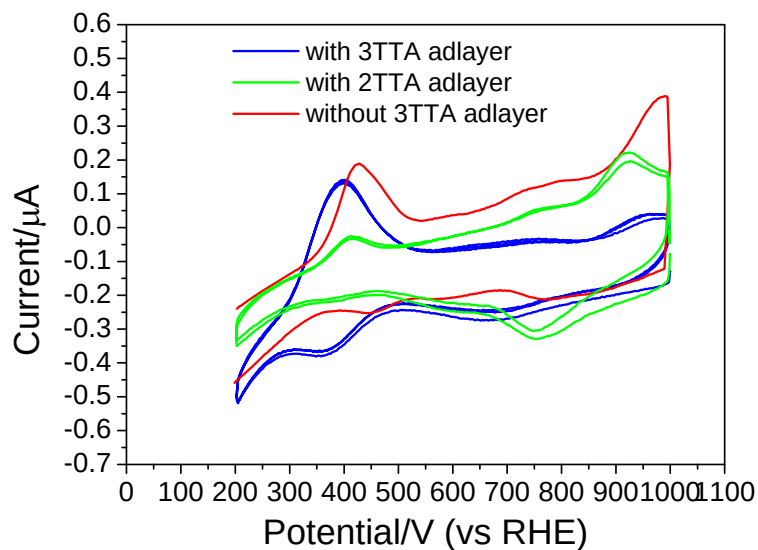
Figure 1. Typical cyclic voltammograms (CVs) of bare Au(111) (red curve), 3TTA-covered Au(111) (blue curve) and 2TTA-covered Au(111) (green curve) electrodes in 0.10 M HClO 4 . The scan rate was 10 mV s -1 .
