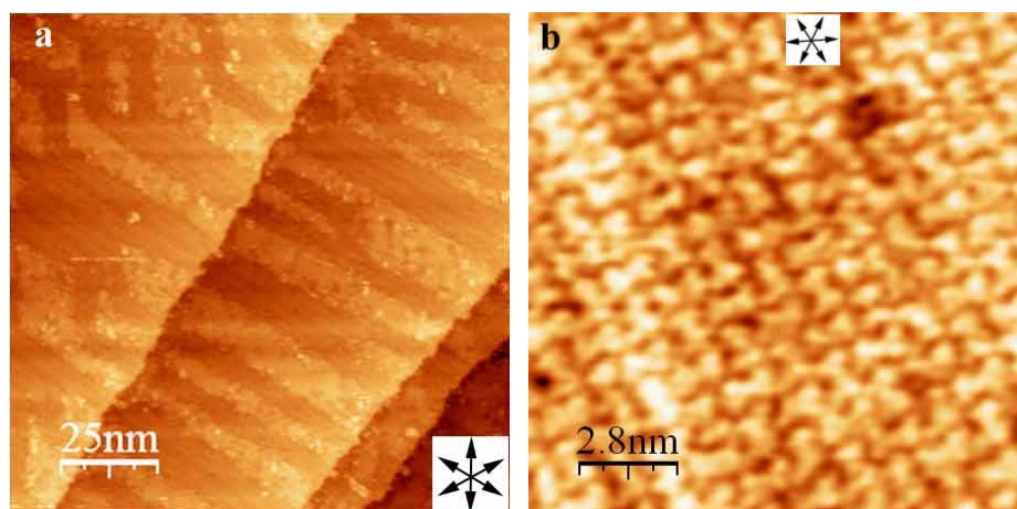
Figure 3. Large scale (a) and high-resolution (b) STM images of 3TTA adlayer on Au(111) acquired in 0.10 M HClO _4 at E = 0.20 V (vs RHE). The bias voltage and the tunneling current were -22 mV and 100 pA, respectively. The set of three arrows indicated the close-packed directions.
