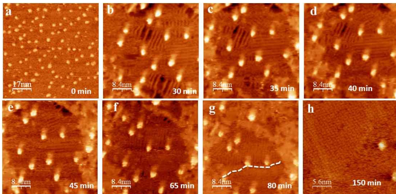
Figure 5. Time-dependent STM images depicting dynamic changes occurring at a monolayer of 3TTA on Au(111) acquired at E=0.20 V (vs RHE) in 0.10 M HClO 4 .
