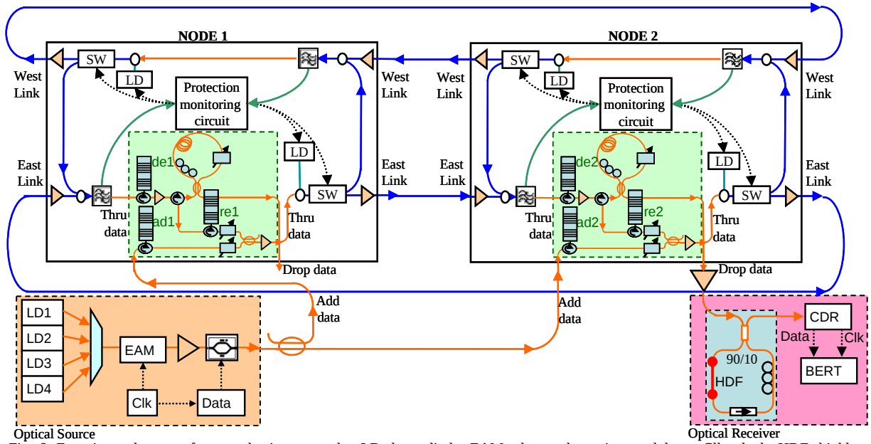
Fig. 6. Experimental setup of two-node ring network. LD: laser diode; EAM: electro-absorption modulator; Clk: clock; HDF: highly GeO 2 -doped fiber; CDR: clock and data recovery unit; BERT: bit-error rate tester.
