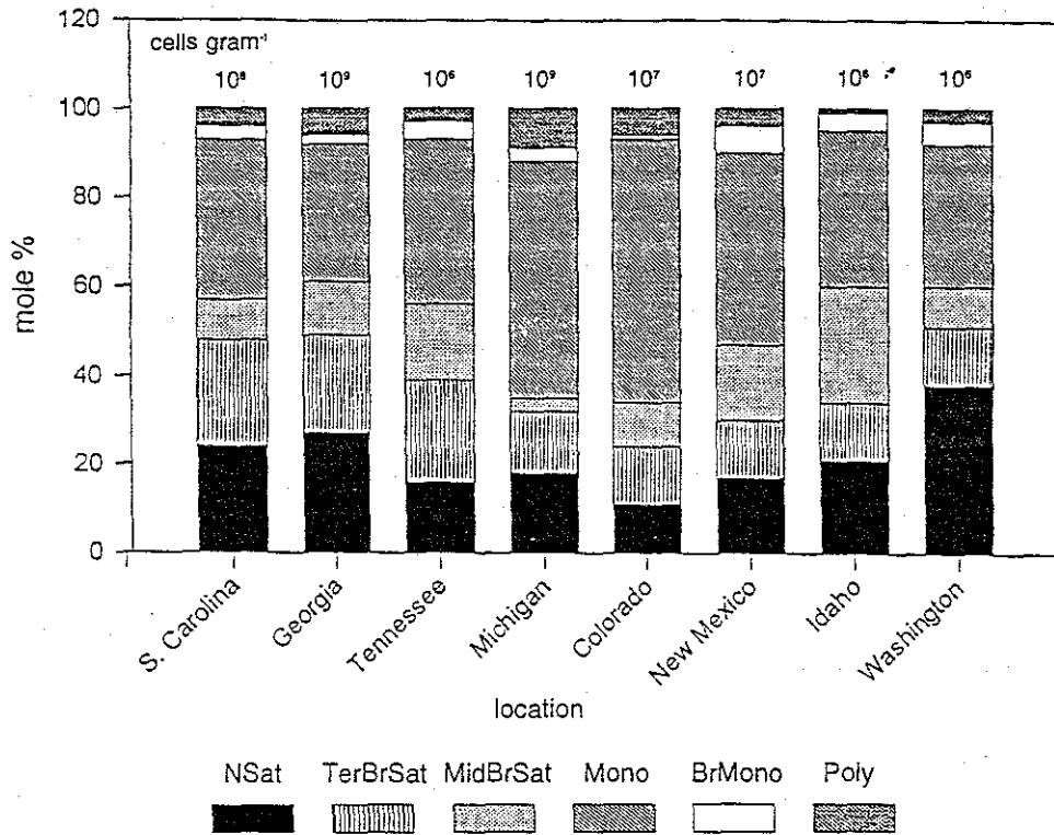
Figure 3 - Viable biomass and community composition from the SLB analyses of surface soils across the USA. Surface soils were recovered from Aiken, SC (22); Decatur, GA; Oak Ridge, TN (24); Upper Peninsula, MI (24); Parachute Creek, CO; Cerro Negro, NM; Idaho Falls, ID; and Richland, WA.
