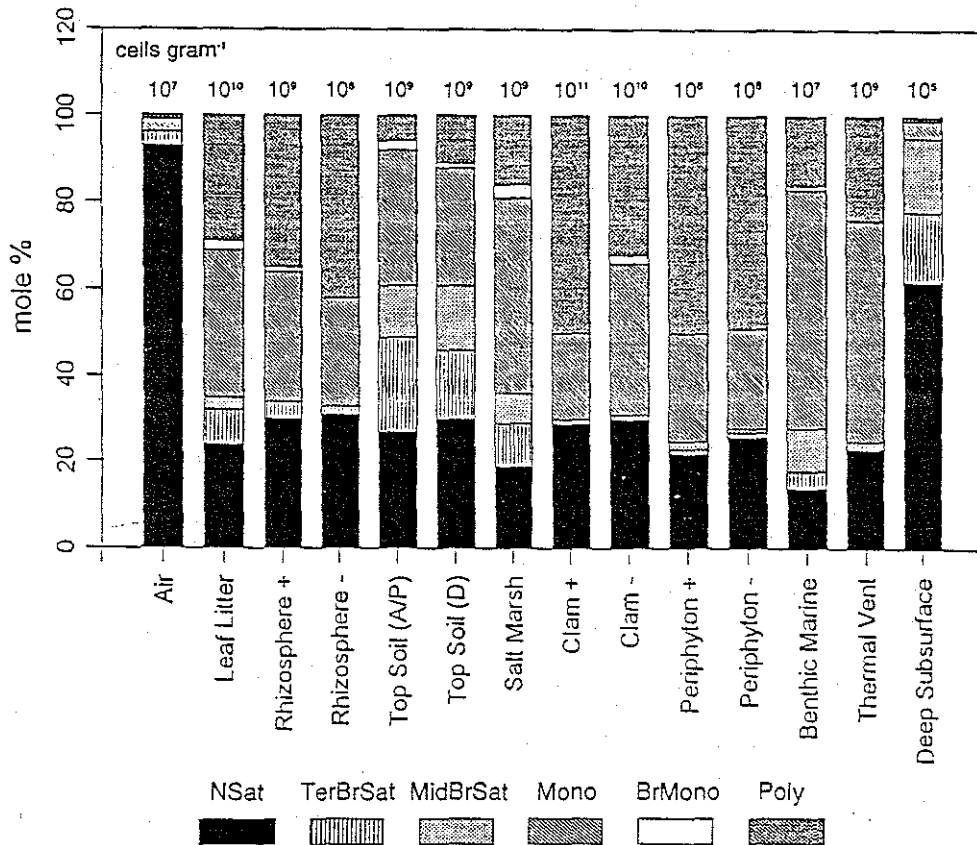
Figure 4 - Viable biomass and community composition from the SLB analysis of selected biomes. Indoor air biocomtaminants collected on a glass fiber from 10 3 m 3 of indoor air; Forest leaf litter from Oak Ridge, TN; Fine root rhizosphere from longneedle pines grown in sand with 400 kg/ha/yr nitrogen and 720 ppm CO 2 (+) compared to the rhizosphere of pines grown with 40 kg/ha/yr nitrogen and ambient CO 2 (-) [324; Surface soils supporting annual and perennial weeds (AVP) versus soils supporting a dimorphic community of sedges (D) near Decatur, GA; Tidal Salt marsh in England (25), Clam Potamocorbula amurensis gills feeding on a phytoplankton bloom (+) versus no bloom (-) (26); Periphyton from freshwater streams (-) compared to the same system impacted by hypochlorite after 30 days of exposure (+) (27); Marine deep sea sediment near Easter Island (208°E at the Equator); Endeavor Ridge hydrothermal vent sediment at 47°57'N, 129°06' W in the Pacific ocean (28); and deep subsurface lacustrine sediment 186 m below the surface at Richmond, WA.
