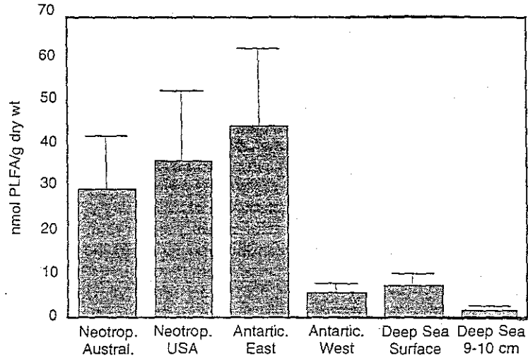
Figure 1 - Viable biomass determined as total PLFA in sandy marine sediments. From left to right: Sand seagrass bed Moreton Bay, Queensland, Australia, top 2 cm of sediment at a 1 m depth, (n = 20) (18); Tidal sea grass estuary in the Gulf of Mexico off Florida, top 1 cm of sediment at a 1 m depth (n = 23) (18); Cape Evans East McMurdo Sound, Antarctica, top 1 cm of sediment at a 35 m depth + 1.5 m of ice (n = 3) (19, 20); Arthur Harbor West McMurdo Sound Antarctica top 1 cm of sediment at a 26 m depth + 2.3 m of ice; Benthic sea bottom top 1 cm (n = 4) (19, 20); Scotian Rise, North Atlantic 40°27'N, 62°20'W at 4820 m depth (n = 48) (21); Scotian Rise, North Atlantic 40°27'N, 62°20'W at 4820 m depth, 9-10 cm below the sediment surface (n = 20) (21).
