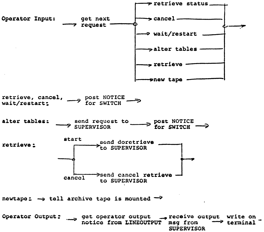
Figure 4.5 Operator Functions
