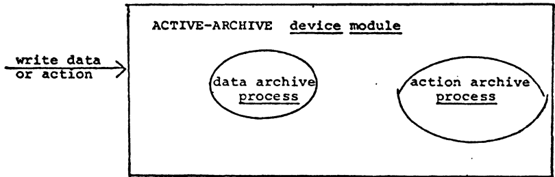
Figure 3.5 Active Archive
