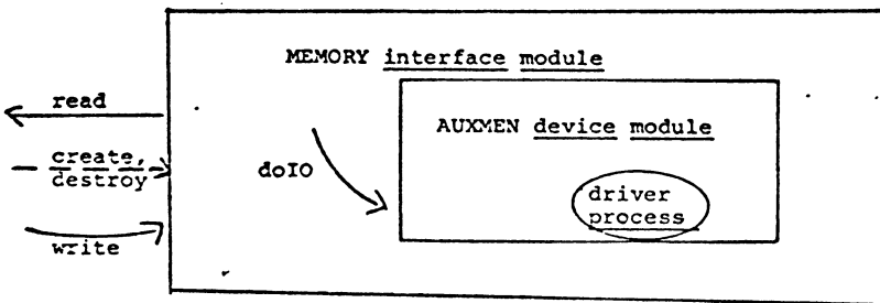
Figure 3.7 Operator
