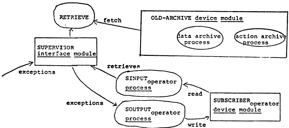
Figure 3.7 Operator
