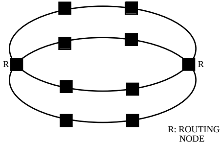
Fig. 4 Symmetrical Multiple-Ring Configuration, n = 2 , N = 4n + 2 = 10
