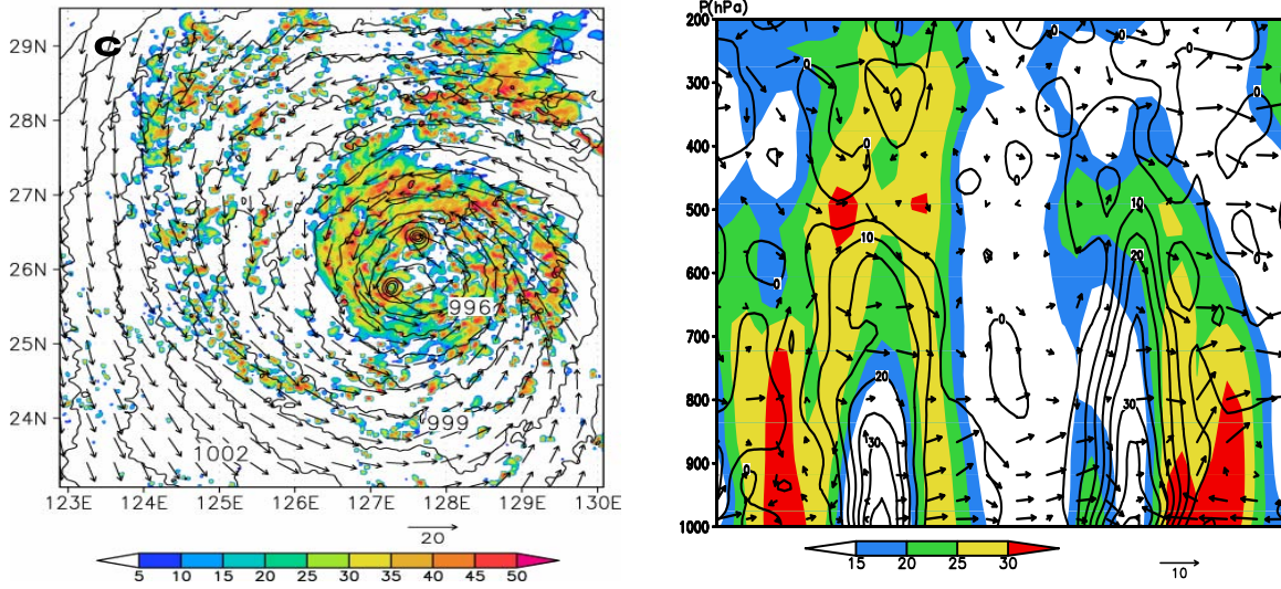
Fig. 2 (a) Horizontal distribution of the simulated radar reflectivity at 900 hPa (shaded), sea-level pressure (solid, every 1 hPa), and surface wind vectors; (b) Vertical cross section of the radar reflectivity (shaded), relative vorticity (solid, every 10^{-4} \text{ s}^{-1} ) and in-plane flow vectors through the two meso- \beta -scale vortices; all from the 60-h simulation of Nari (2001).
