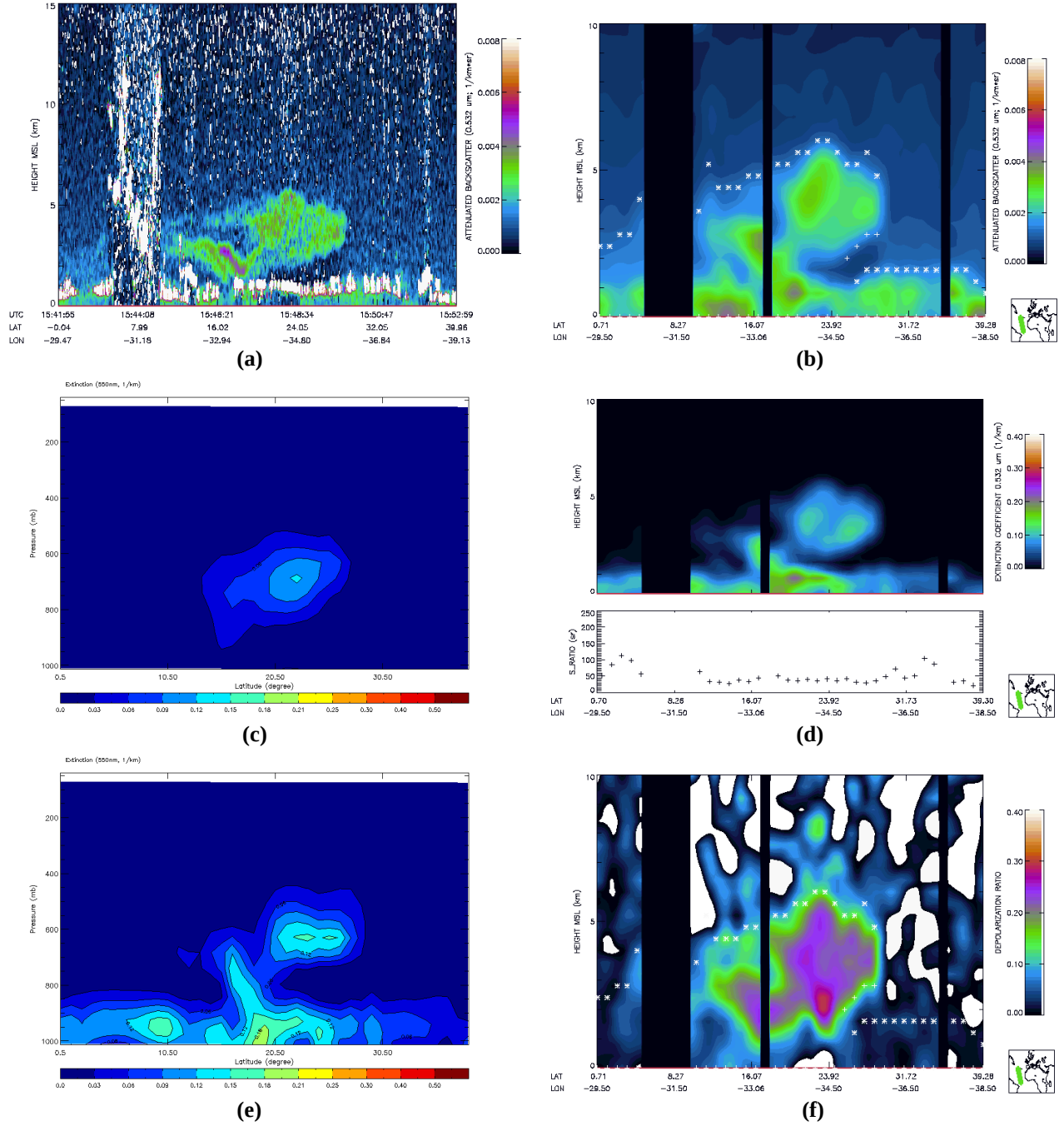
Figure 1. (a) CALIOP 0.532 \mu\text{m} attenuated backscatter ( \text{km}^{-1} \text{sr}^{-1} ) for 1522 UTC orbital pass 20 July 2007, 0^\circ to 40^\circ N from 0.0 to 15.0 km MSL; (b) 1^\circ along-track gridded attenuated backscatter profiles from 0.0 to 10.0 km MSL; (c) NAAPS analysis of extinction coefficient ( \text{km}^{-1} ) from 1000.0 to 100.0 hPa for this pass using only MODIS/MISR optical depth assimilation; (d) 0.532 \mu\text{m} extinction coefficient and extinction-to-backscatter ratios for inversion constrained by NAAPS optical depths in (c); (e) NAAPS extinction coefficient ( \text{km}^{-1} ) post-CALIOP assimilation; (f) 0.532 \mu\text{m} CALIOP 1^\circ along-track linear depolarization ratio. Derived aerosol layer boundaries are denoted by asterisks (top) and plus symbols (bottom), respectively.
