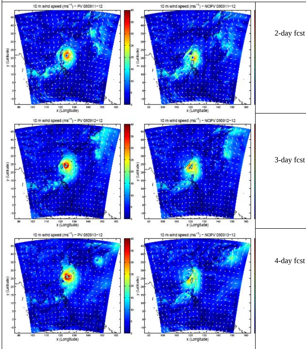
FIGURE 2. Left column: WRF forecast for Typhoon Sinlaku initialized on 12 UTC, 09 September 2008. Right column: As for the left column, but with the shortwave removed from the initial conditions.
