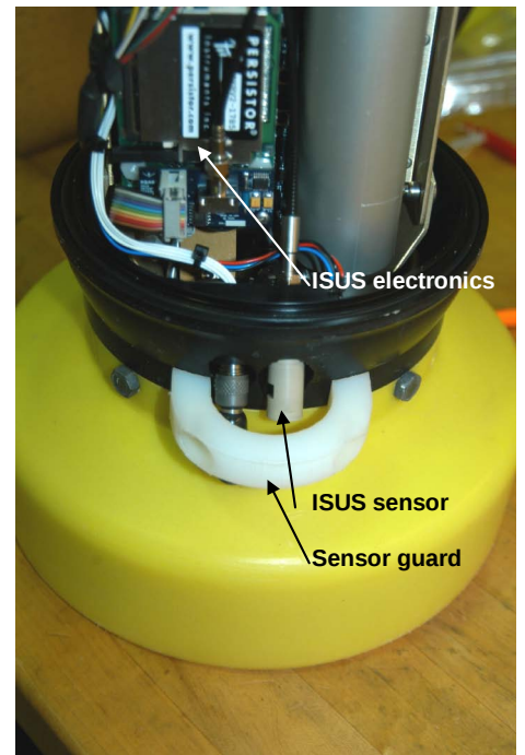
FIGURE 1. The initial design of ISUS for a profiling float. In this version the sensor is located on the lower endcap of the float. The float is also equipped with an Aanderaa Optode dissolved oxygen sensor and uses Iridium communications.
