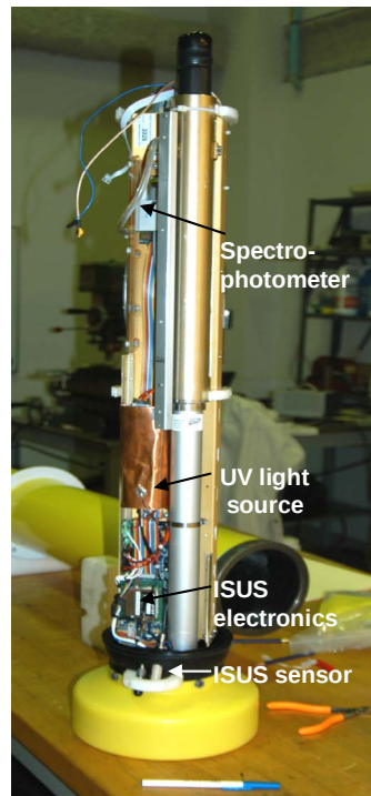
FIGURE 1. The initial design of ISUS for a profiling float. In this version the sensor is located on the lower endcap of the float. The float is also equipped with an Aanderaa Optode dissolved oxygen sensor and uses Iridium communications.
