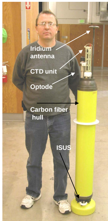
FIGURE 1. The initial design of ISUS for a profiling float. In this version the sensor is located on the lower endcap of the float. The float is also equipped with an Aanderaa Optode dissolved oxygen sensor and uses Iridium communications.
