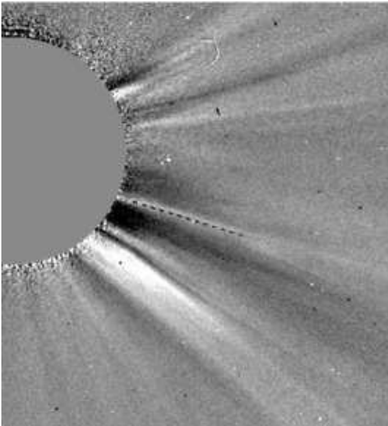
Fig. 9. Determining excess masses (densities) along the ray (dashed line) from the COR2A observation at 17:52:20 UT. A pre-event frame taken at 09:22:00 UT was subtracted.
