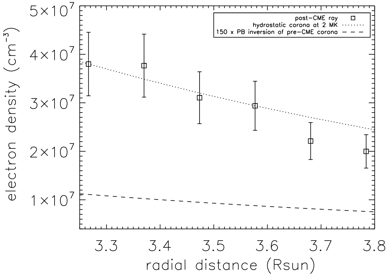
Fig. 10. Density along the ray as a function of heliocentric distance (squares). Density profile of the pre-CME corona on 9 April 2008, 10:06 UT from LASCO C2 PB data inversion (dashes). Density distributions for a hydrostatic isothermal corona at 2 MK (dots).
