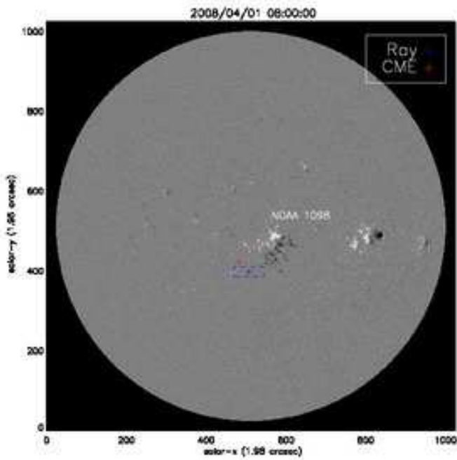
Fig. 11. Overlay of the CME (red cross) and ray (blue cross) central longitudes and latitudes determined from the 3D modeling of Section 3 on an MDI magnetogram taken during 1 April 2008, when the host AR (i.e., NOAA 1098) was close to the central meridian as viewed from SOHO. The dashed blue box has a length/height equal to the depth/thickness of the WL ray as determined from our 3D modeling. Its orientation cannot not be determined from our modeling (see the discussion of Section 3).
