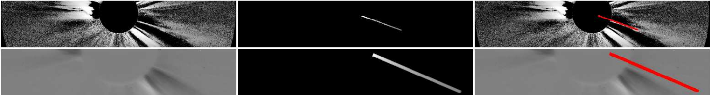
Fig. 8. Same as in Fig. 7 but for a ray model with twice the depth and the thickness of that of Fig. 7.
