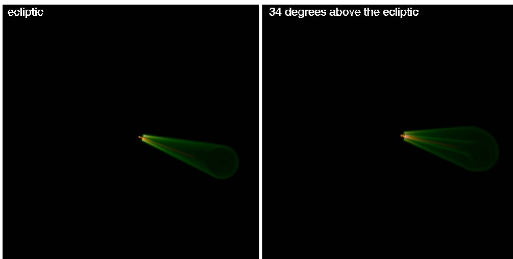
Fig. 12. Combined TB view of the CME (green) and of the ray (orange). View from the ecliptic plane (left panel). View 34 degrees above the ecliptic plane (right panel). Both views are from a distance of 100 R_{\odot} .
