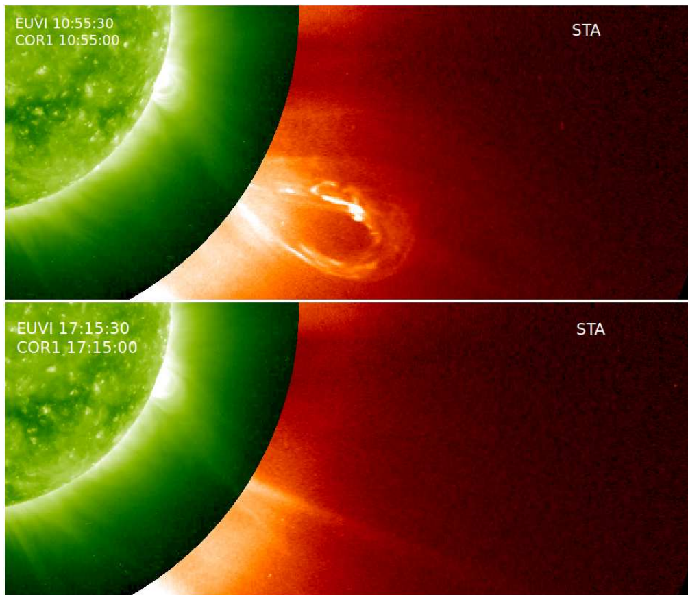
Fig. 1. Composite of EUVI-A 195 (inner FOV) and COR1-A (outer FOV) showing the emerging CME (upper panel) and the resulting WL ray (lower panel). The temporal evolution is shown by movie1.mpg.
