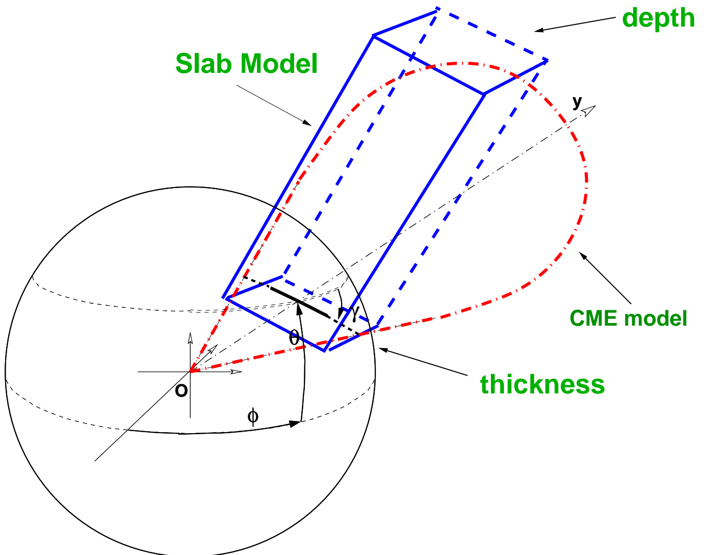
Fig. 4. Schematic of the 3D models used in the modeling of the WL CME (red) and ray (blue).
