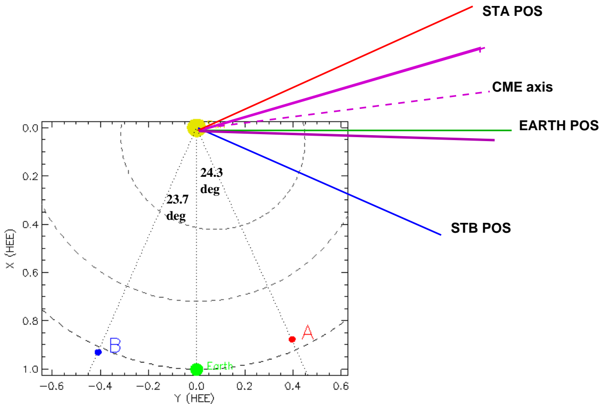
Fig. 6. Schematic of the orientation (dashed magenta line) and of the angular width of the CME (solid magenta lines) as determined from the 3D modeling of Section 3. The plot also supplies the relative positions of STB, Earth and ST as well as the corresponding POS (blue, green and red solid lines respectively) during 9 April 2008.
