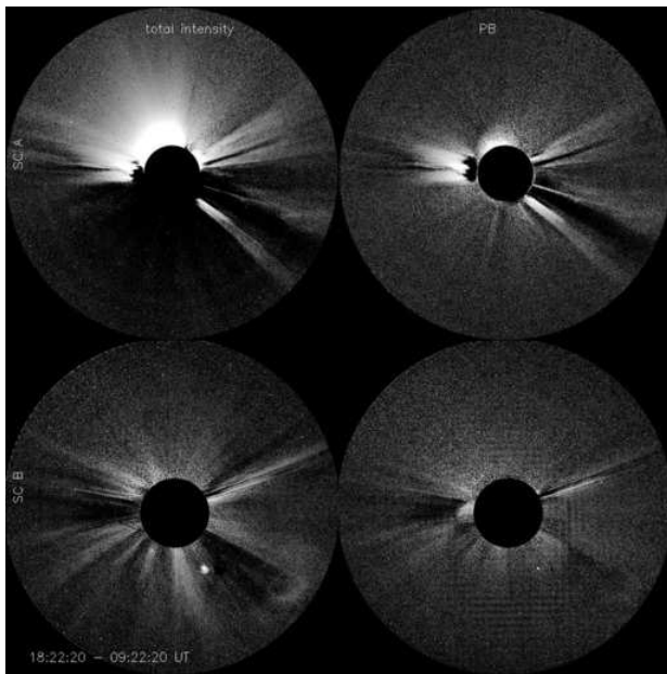
Fig. 3. TB and PB images for STA (first row) and for STB (second row). They were taken at 18:22:20 UT. Pre-event TB and PB images were subtracted. Field of view spans from 2.5 - 15 R_{\odot} .
