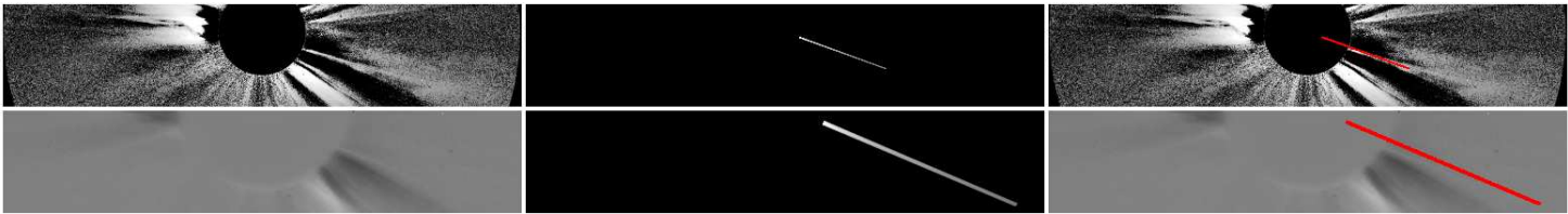
Fig. 7. 3D geometrical modeling of the ray observations of STA/COR2 (upper panel) and of LASCO/C2 (lower panel). The left column shows TB images for each spacecraft, where a pre-event image was first subtracted. The middle column shows TB images of the ray from our 3D modeling whereas the right column shows overlays of the rectangular slab model wireframe (red) on the corresponding TB images. Times of the observation: 17:52:20 UT for STA/COR2 and 17:50:04 for LASCO/C2.
