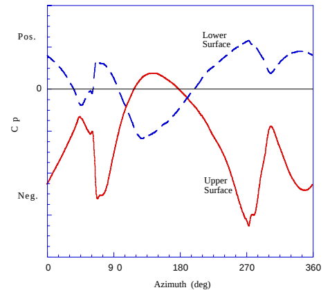
b) Upper and Lower c_p time histories for x/c = 3.5\%
