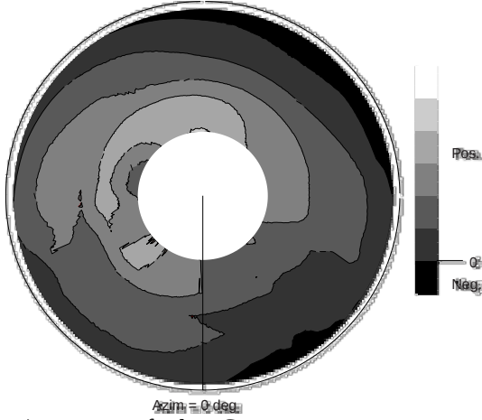
a) c_N contour for low C_T .
