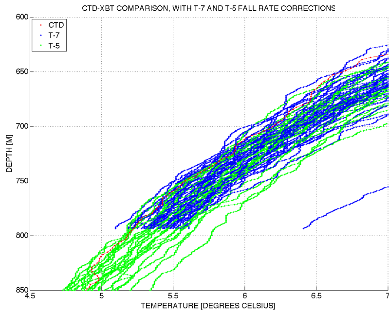
Figure 10b. Corrected PhilSea09 XBT data. T5 (green) and T7 (blue) XBT temperature data vs. depth corrected for fall rate. CTD data (red).
