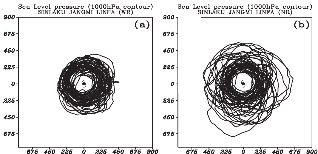
FIG. 16. 1000-hPa contours of sea level pressure analyzed relative to typhoon center (typhoon symbol) from 52 cases of (a) WR and (b) NR experiments (axis units in km).
