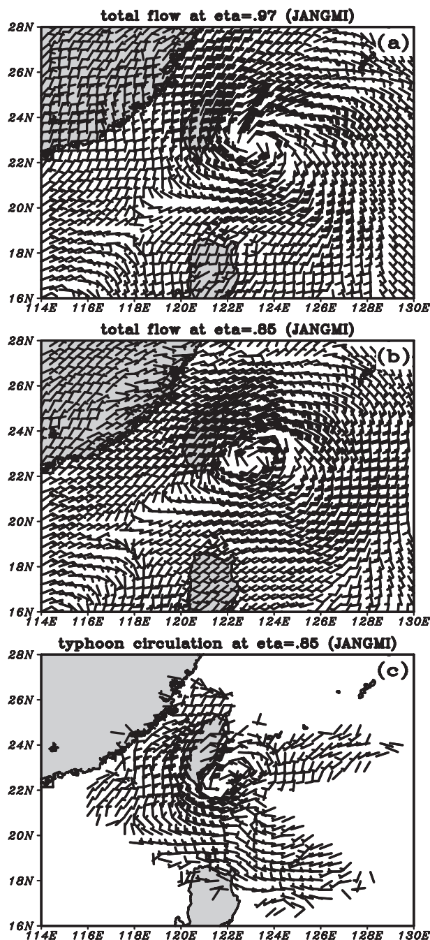
FIG. 4. Low-level wind distorted by Taiwan terrain as Typhoon Jangmi approaching Taiwan at 0000 UTC 28 Sep 2008 at (a) \eta = 0.97 level, (b) \eta = 0.85 level, and (c) extracted typhoon circulation at \eta = 0.85 level.
