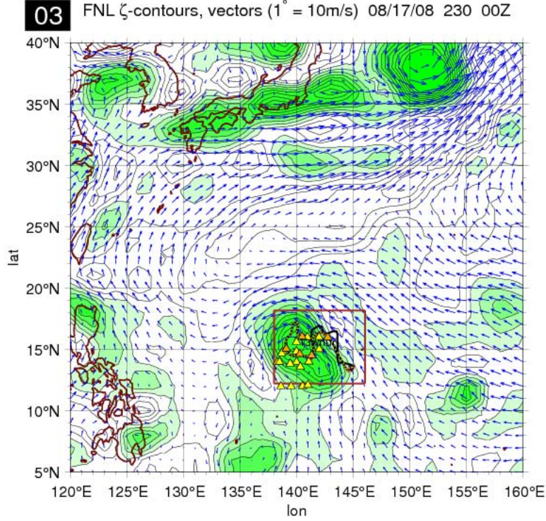
Figure 1: Vorticity and winds from the NCEP FNL analysis with P-3 aircraft track and P-3 and C-130 dropsonde locations overlayed.
