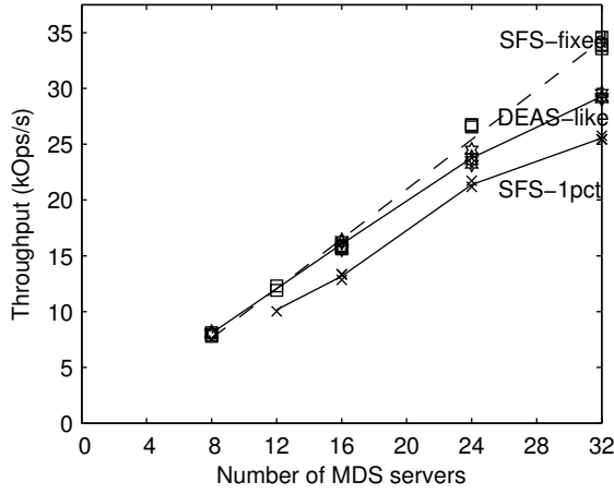
(a) Large constellation MDS throughput
