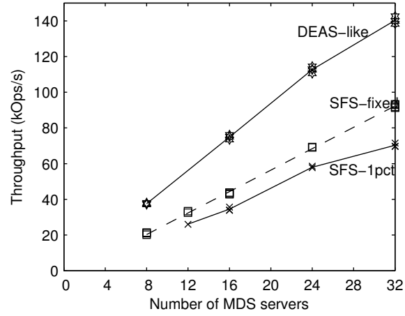
(b) Large constellation NFS throughput
