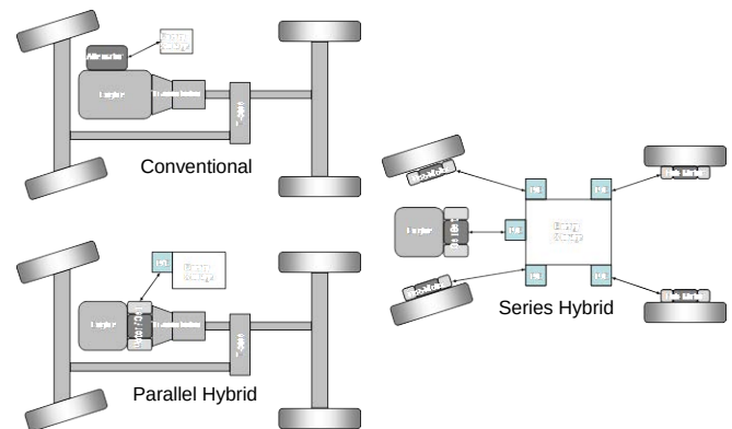
Figure 3: Baseline powertrain architecture alternatives for FED
