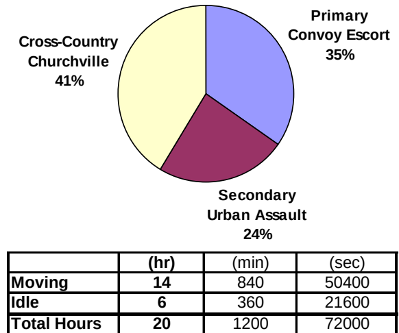
Figure 2: Usage cycle defined for the Fuel Efficient Demonstrator Program
