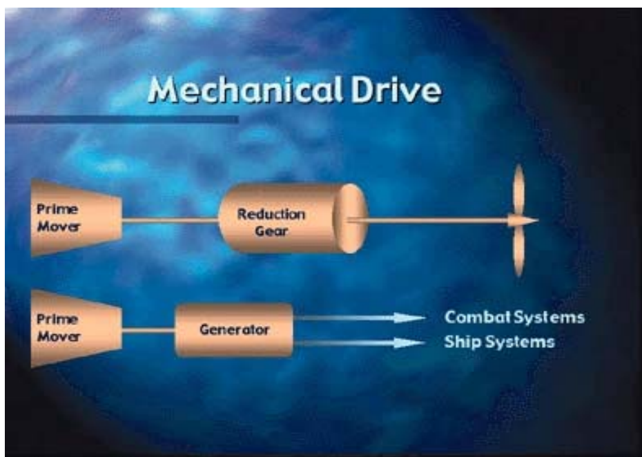
Figure 1. Mechanical Ship. From [1].
