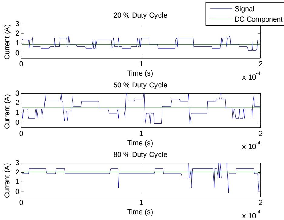
Digital Waveforms in FGPA. 30 kHz Signal.
