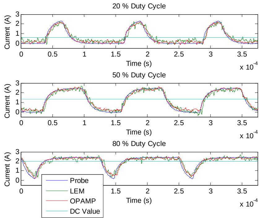
8 kHz Test Results. DC Value is the DC Component of OPAMP Signal
