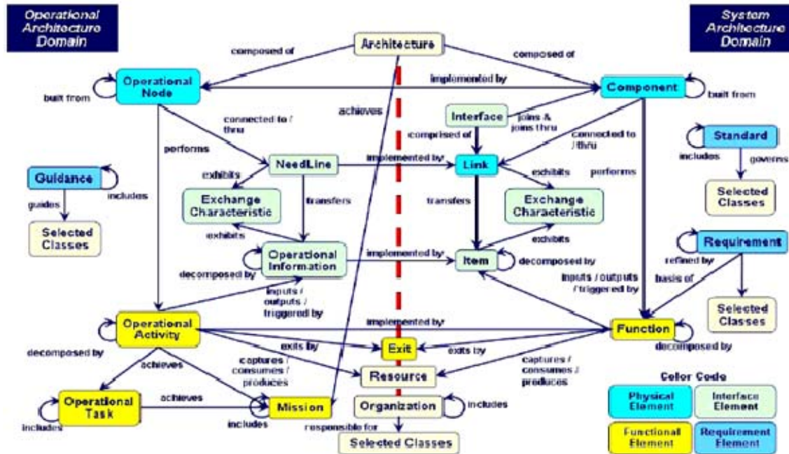
Figure 6. CORE ® DoDAF V1.5 architecture composition. This perspective divides the architecture into two domains: operational and system. (From Vitech, 2007, p. vii)
