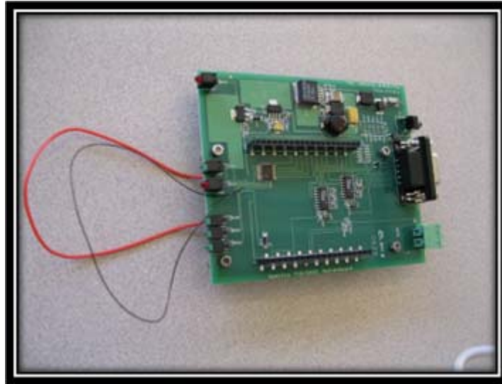
Figure 22. MHX2400 Modified Development Board
