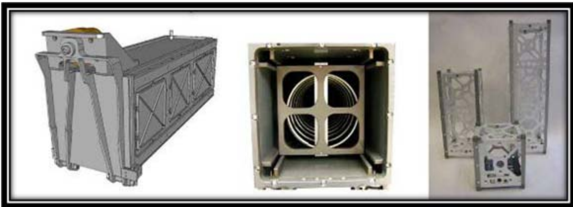
Figure 1. P-POD and CubeSat Structures: 2U, 1U, 3U (From [2])
