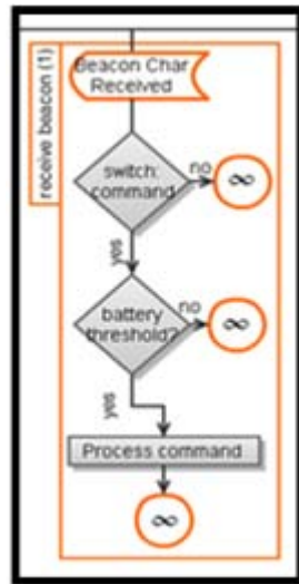
Figure 13. Receive Beacon Task
