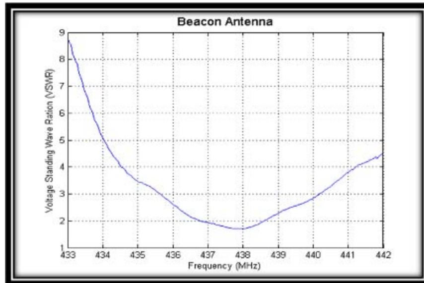
Figure 42. Beacon Antenna Voltage Standing Wave Ratio
