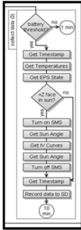
Figure 8. Collect Data Task
