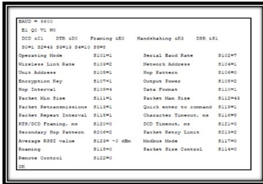
Figure 25. MHX2400 AT Command Interface (From [20])
