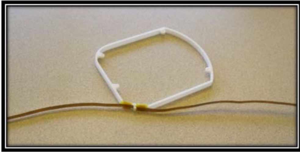
Figure 37. First Beacon Antenna Design with Beryllium Copper
