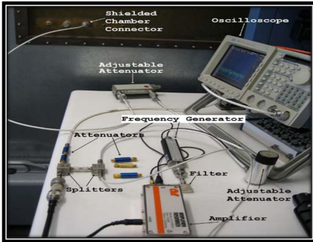
Figure 28. Beacon Carrier-To-Noise Test Oscilloscope, Attenuators, Splitters, Amplifiers, Power Supplies and Frequency Generator
