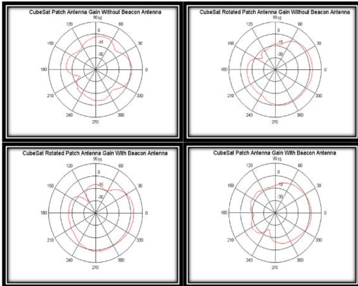
Figure 36. Patch Antenna Gain Patterns
