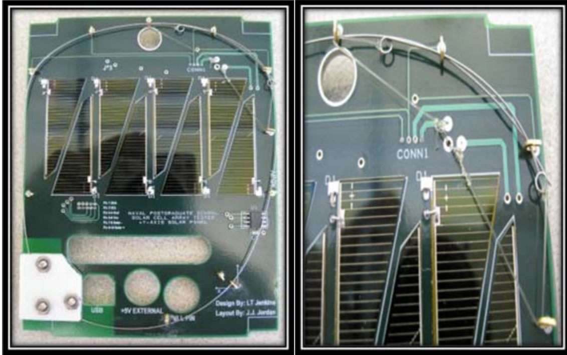
Figure 40. Beacon Antenna Storage Setup
