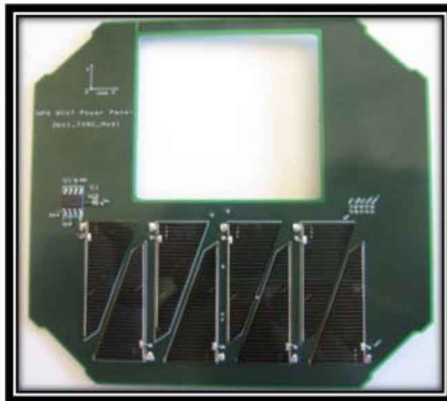
Figure 31. +z Solar Panel With Patch Antenna Cutout
