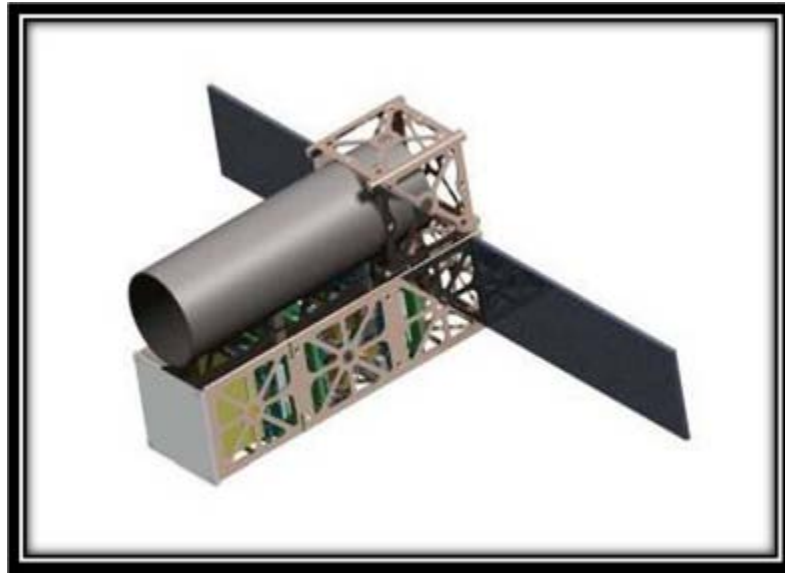
Figure 4. TINYScope CubeSat Concept (From [2])
