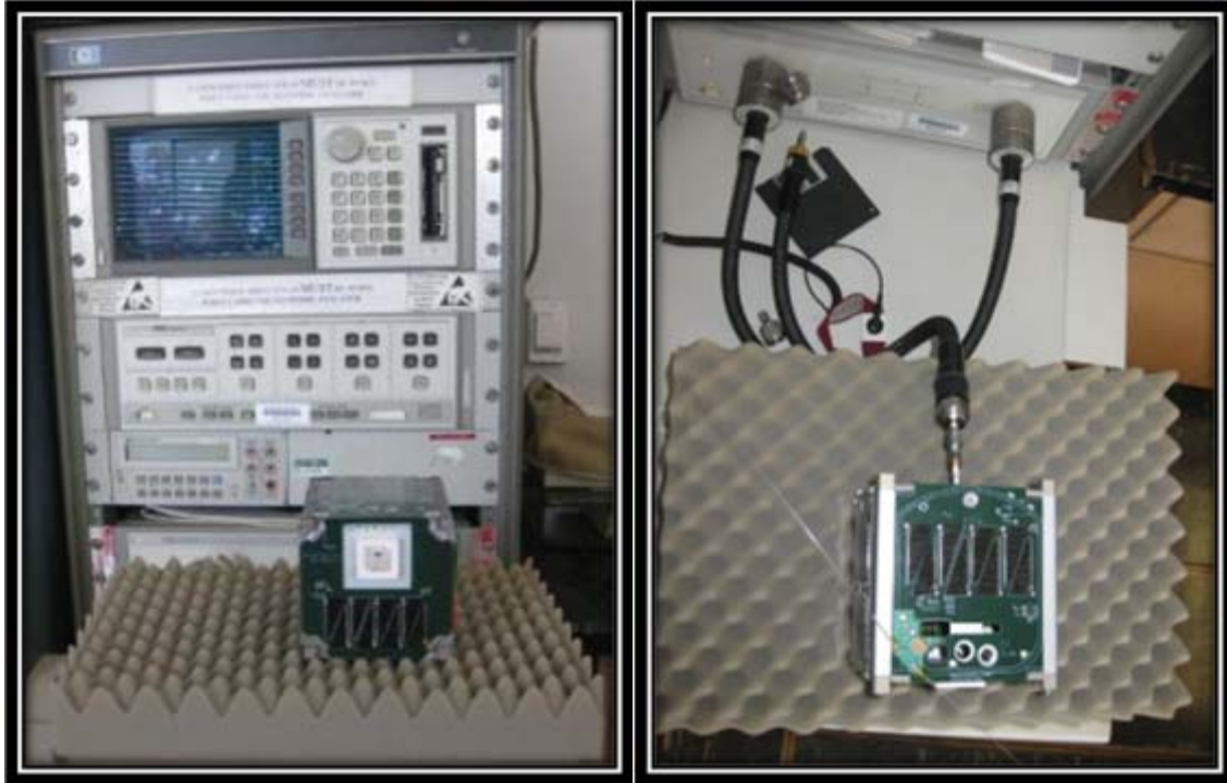
Figure 33. Voltage Standing Wave Ratio Testing
