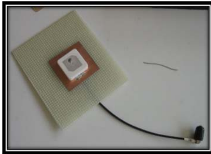
Figure 29. NPS-SCAT Primary Radio Patch (After [7])
