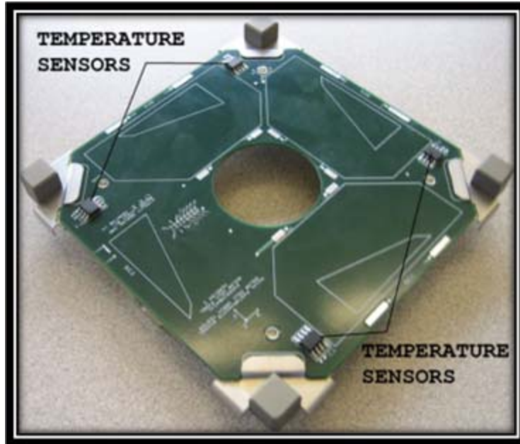
Figure 17. Temperature Sensors
