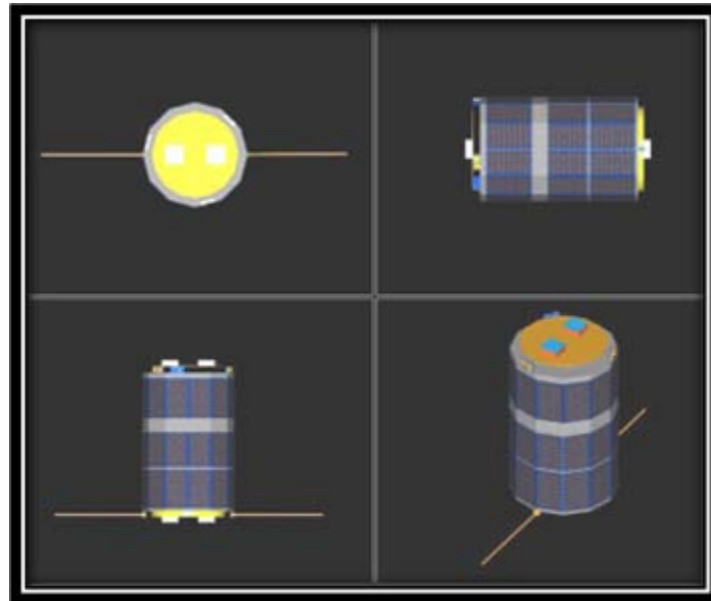
Figure 3. Computer Generated Model of NPSAT1 (From [13])
