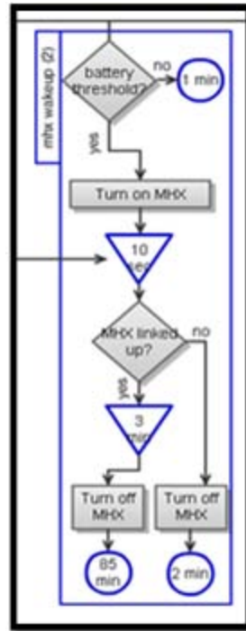
Figure 9. MHX Wakeup Task
