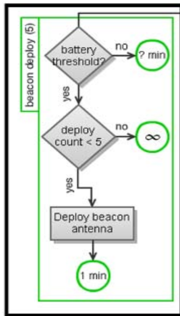
Figure 7. Beacon Antenna Deploy Task
