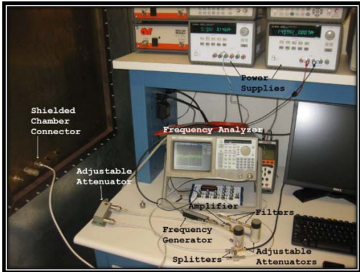
Figure 24. MHX2400 Carrier-To-Noise Test Oscilloscope, Attenuators, Splitters, Amplifiers, Power Supplies and Frequency Generator
