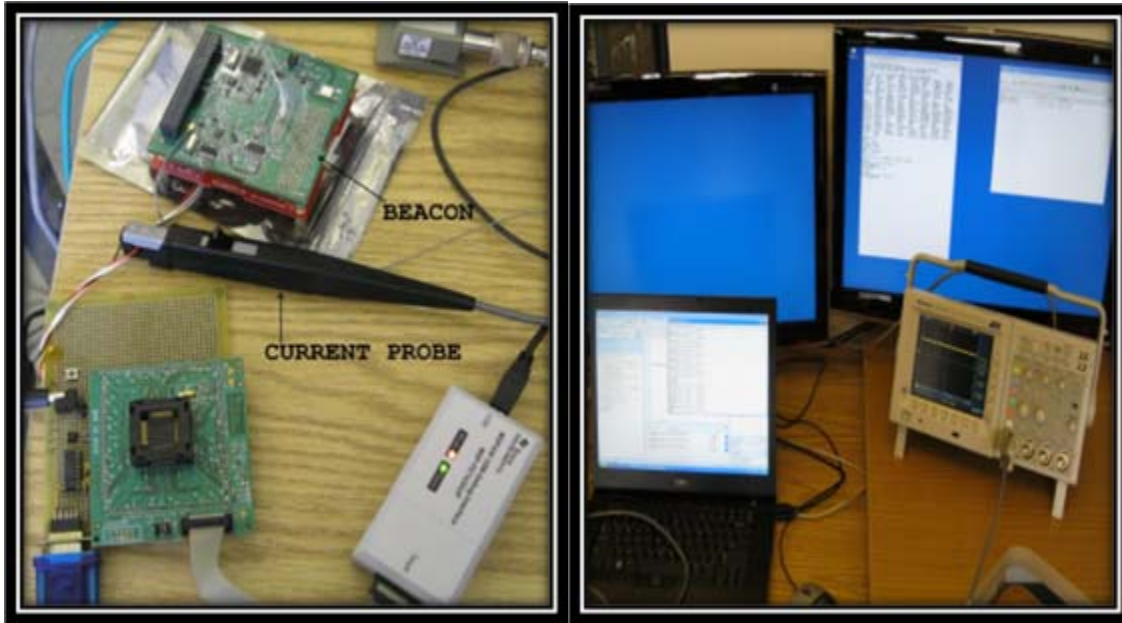
Figure 26. Beacon Current Draw Test
