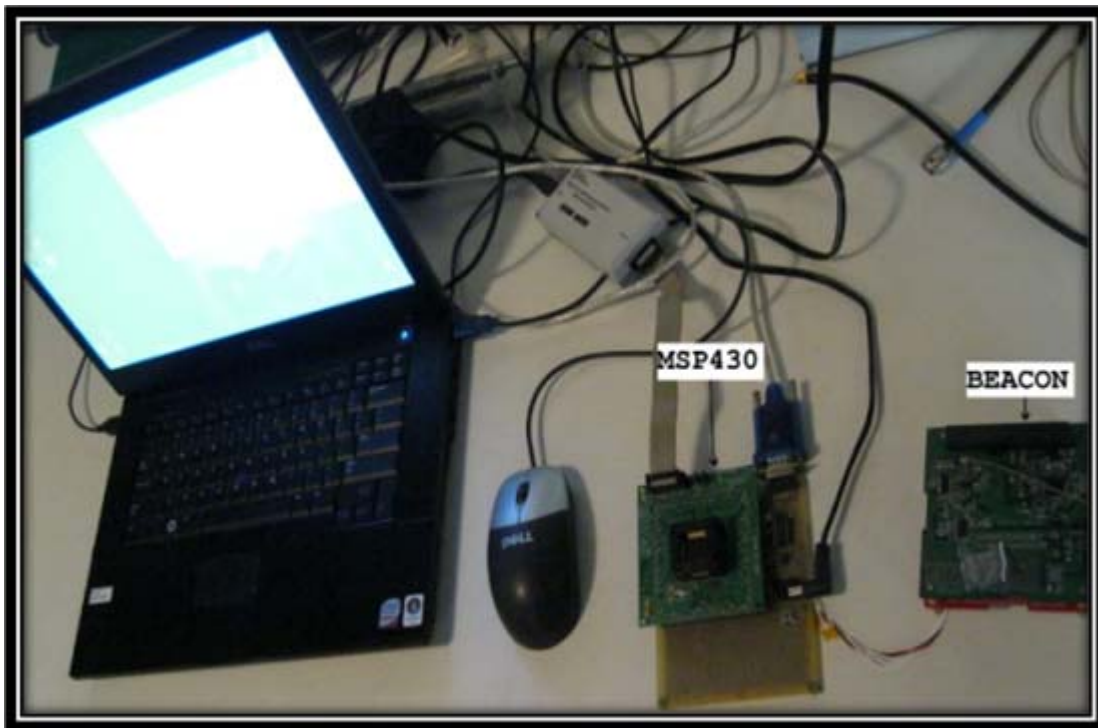
Figure 27. Beacon Carrier-To-Noise Test Setup Inside Shielded Chamber
