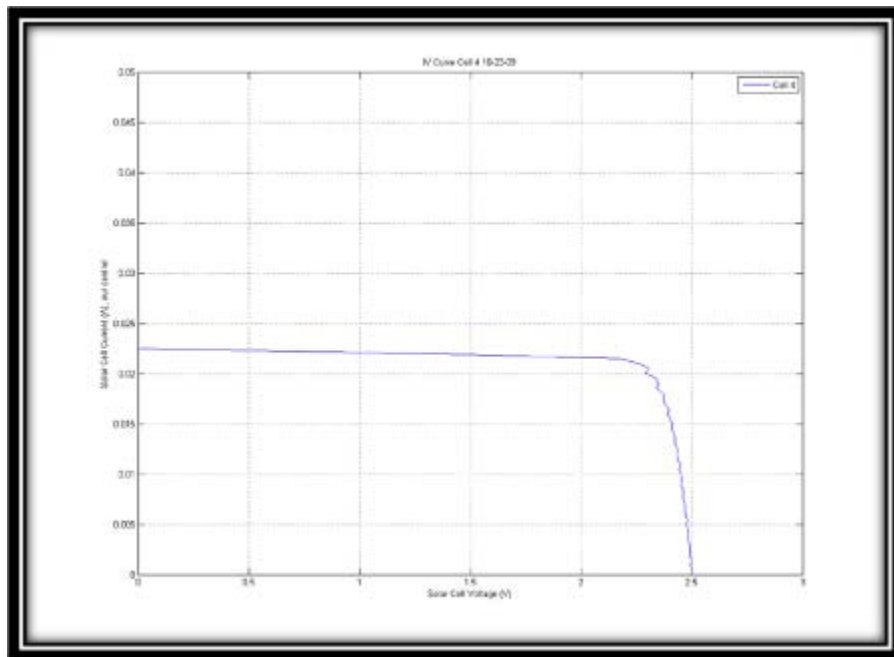
Figure 15. Example I-V Curve
