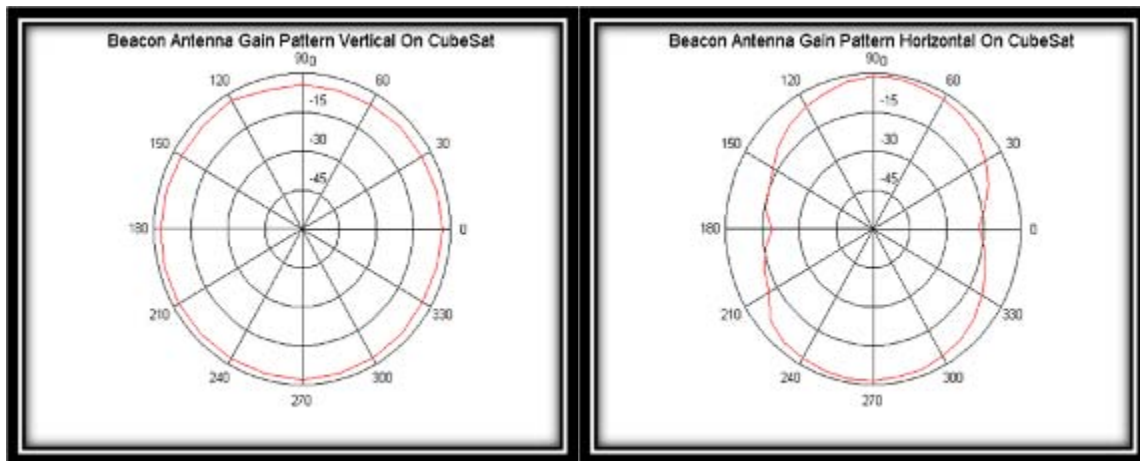
Figure 44. Beacon Antenna Gain Pattern
