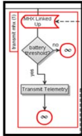
Figure 10. Transmit MHX Task
