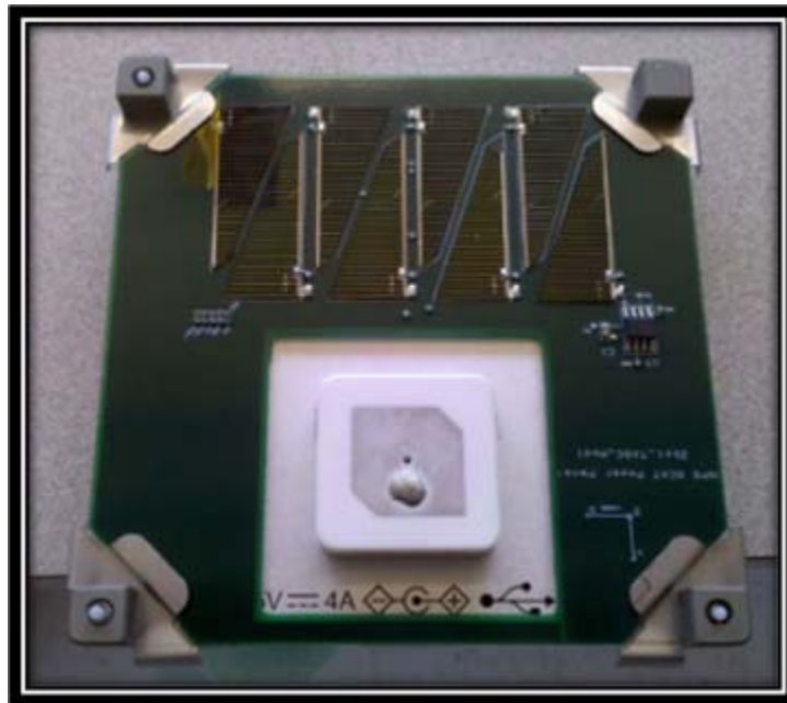
Figure 32. Patch Antenna Attached To CubeSat Structure
