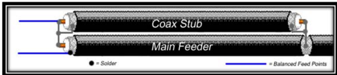
Figure 39. Pawsey Stub Balun (From [29])
