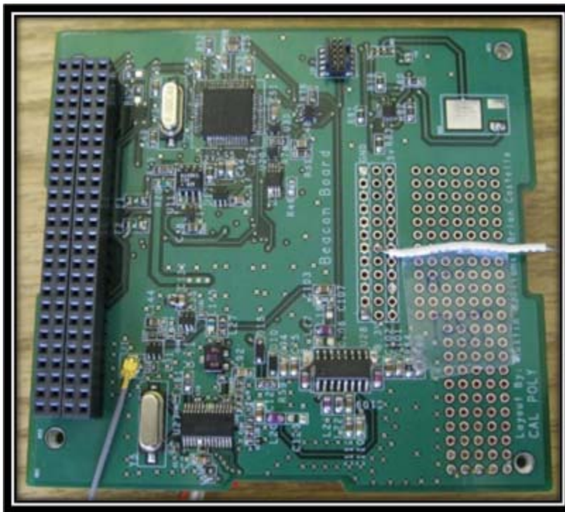
Figure 20. Beacon (UHF Transceiver)
