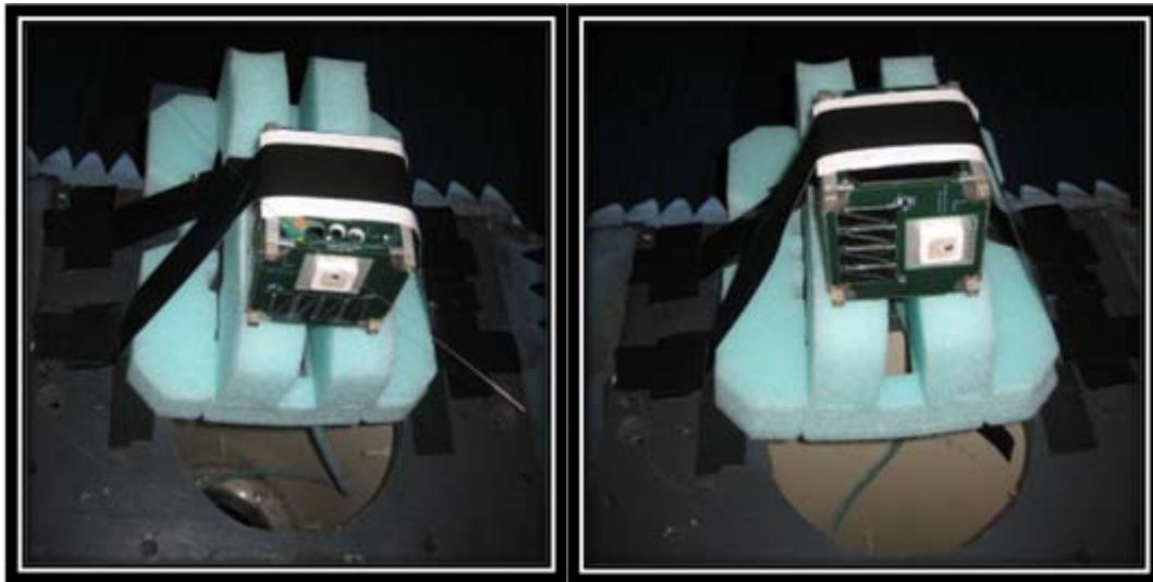
Figure 35. Patch Antenna Anechoic Chamber Test Setup
