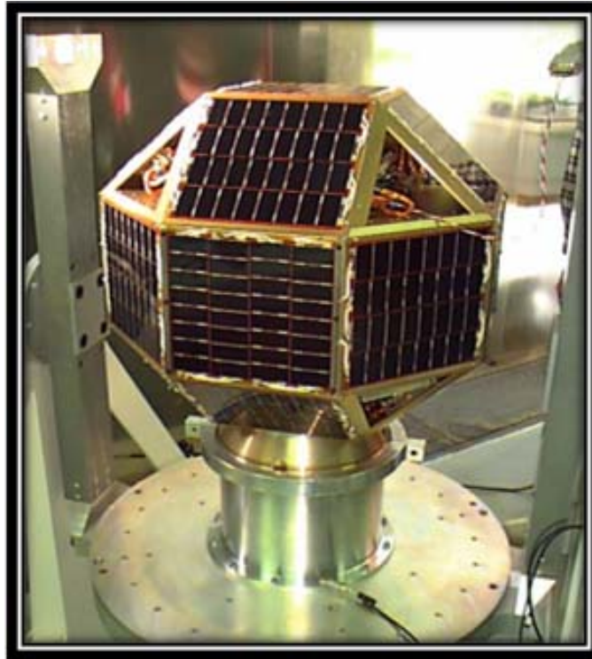
Figure 2. PANSAT During Testing
