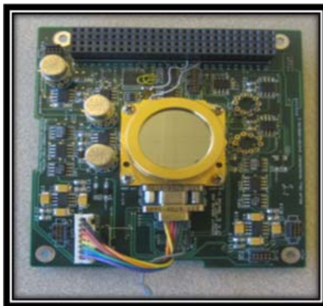
Figure 14. Solar Cell Measurement System (SMS)
