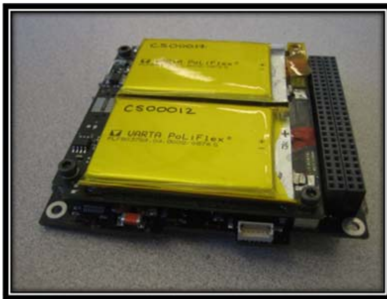
Figure 16. Electrical Power System with Batteries
