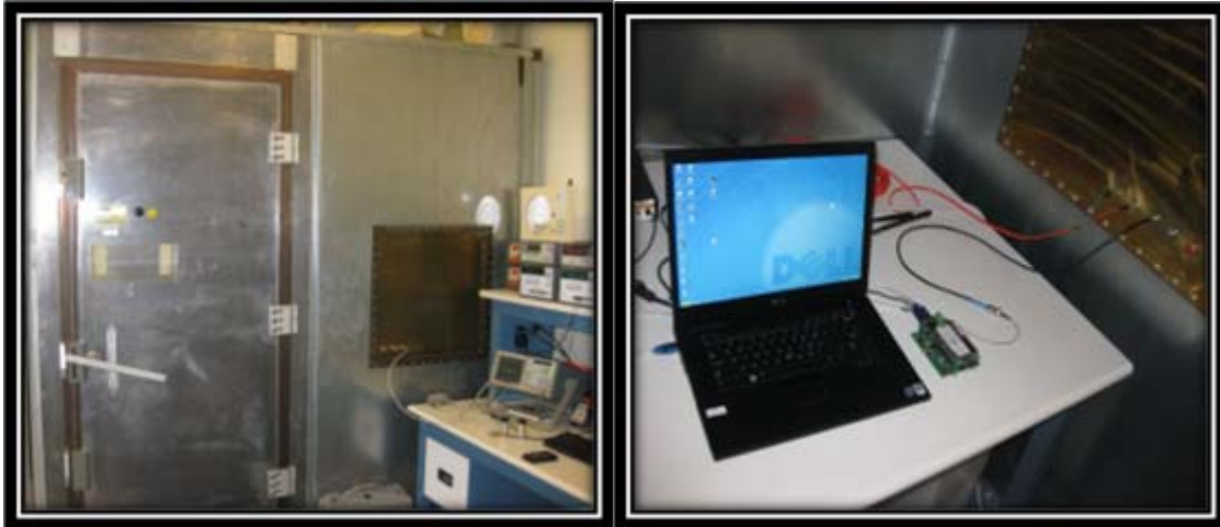
Figure 23. MHX2400 Carrier-To-Noise Test: Shielded Chamber (left) and Inside Shielded Chamber (right)
