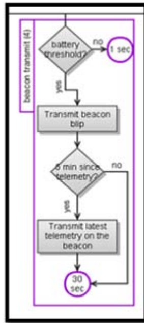
Figure 12. Beacon Transmit Task
