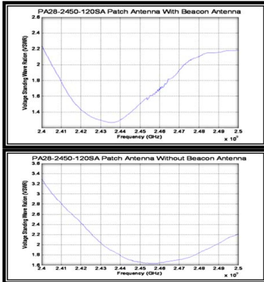
Figure 34. Patch Antenna VSWR Plots
