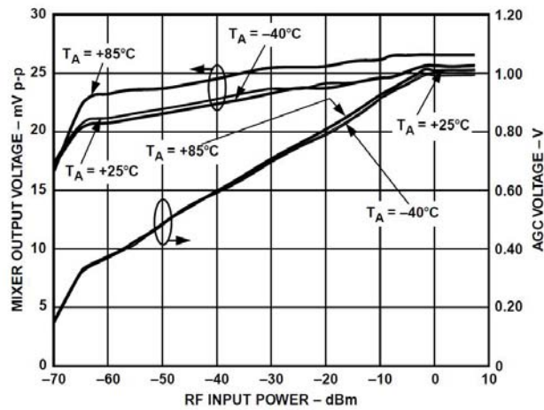
Figure 50. AD8947 AGC voltage and mixer output level vs. RF input power, F_{LO}=1900\text{ MHz} , F_{BB}=1\text{ MHz} , V_S=5\text{ V} (From [13]).
