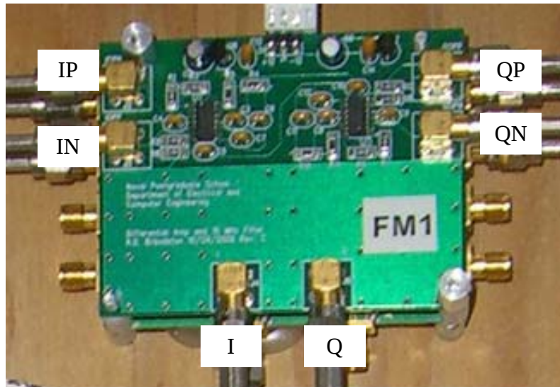
Figure 42. Supplementary amplifier board (After [12]).
