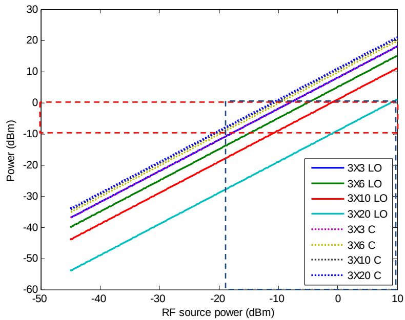
Figure 54. Coupler selection result ( X = 3 dB).
