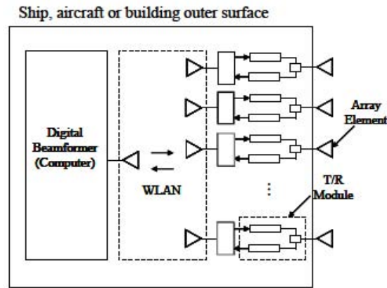
Figure 4. Diagram of a WDDPA (From [3]).
