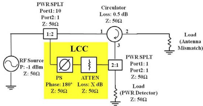
Figure 16. DBFC with modified antenna configuration.
