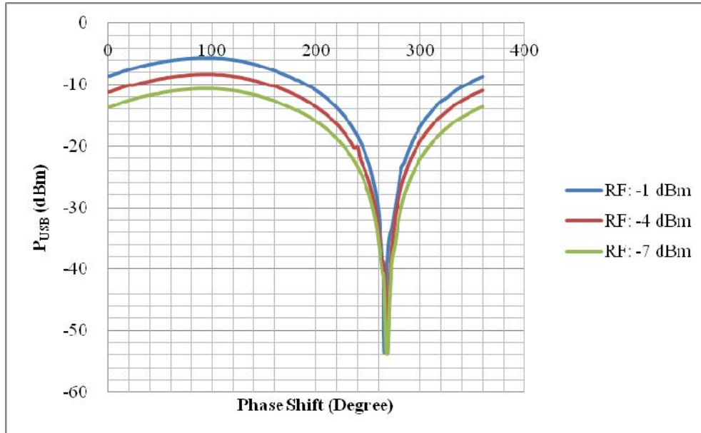
Figure 33. LCC measured result (with digital attenuator).
