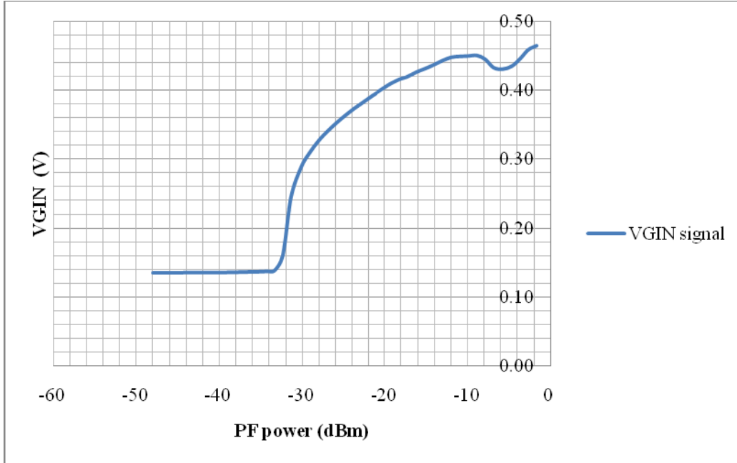
Figure 52. VGIN voltage curve.
