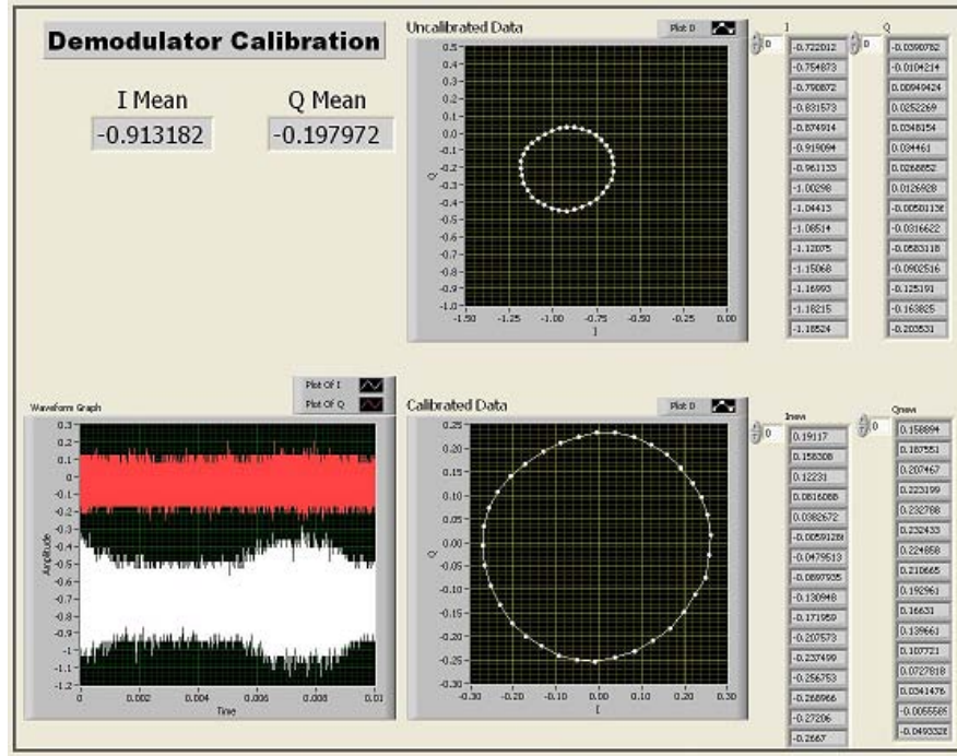
Figure 47. Demodulator calibration result.
