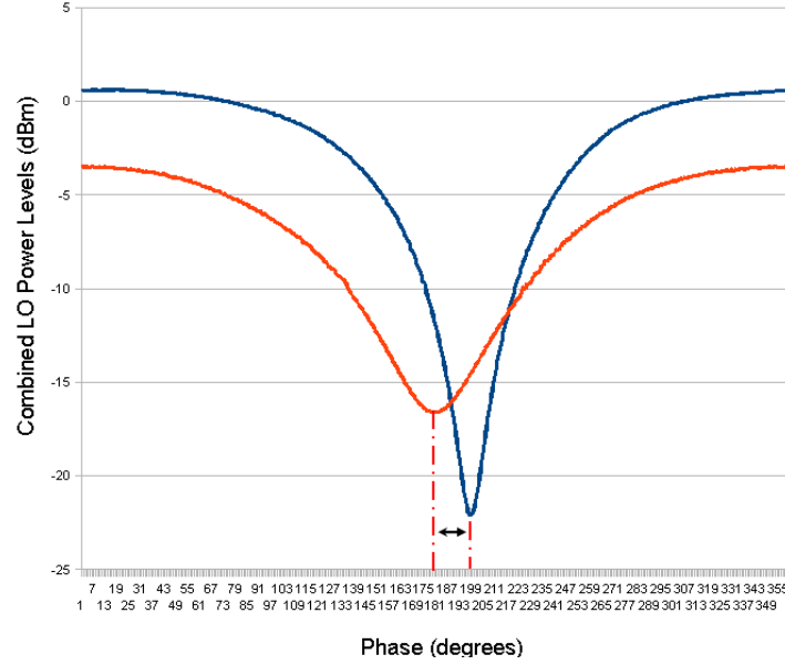
Figure 9. A comparison of synchronization data before (red) and after (blue) incorporating the LCC (From [4]).
