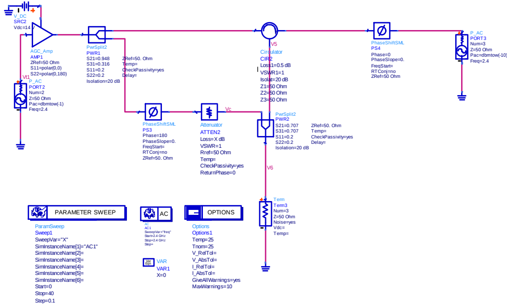
Figure 10. Example of an ADS circuit design schematic.
