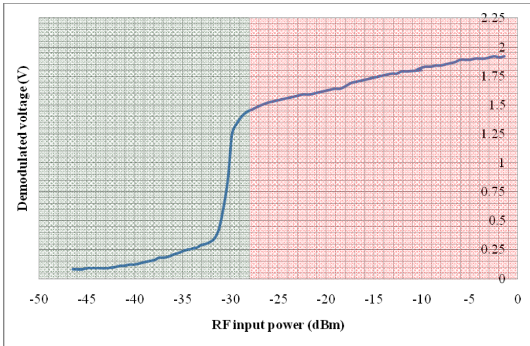
Figure 49. Demodulator dynamic range.
