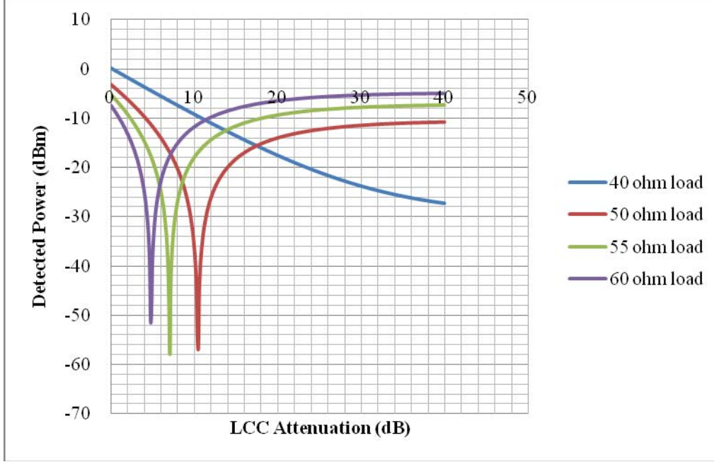
Figure 17. Simulation under different load impedances simulating antenna mismatch.
