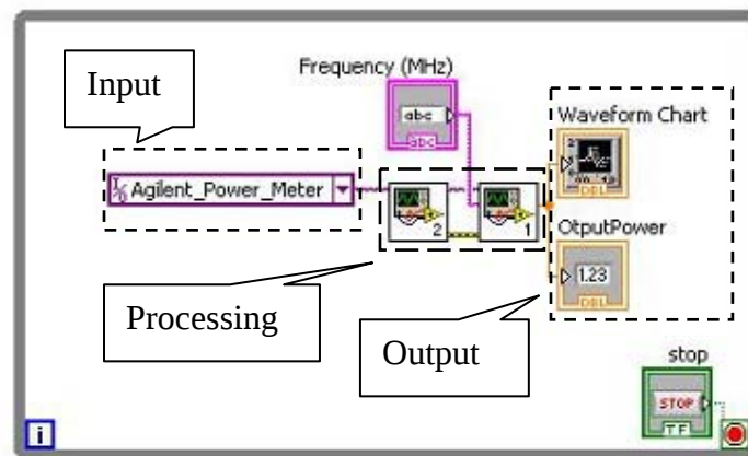
Figure 29. Power measurement block diagram.
