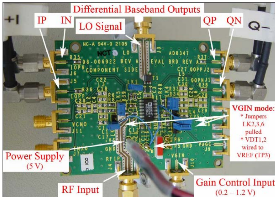
Figure 41. AD8347 demodulator board (From [12]).
