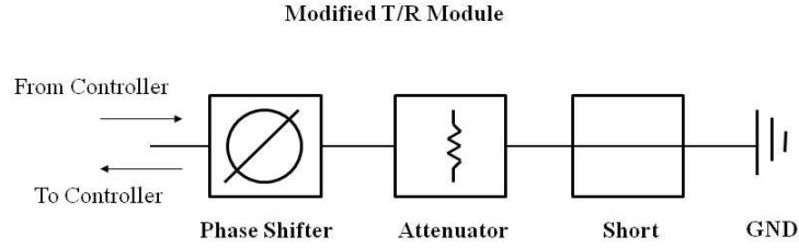
Figure 19. Modified TRM including propagation path.
