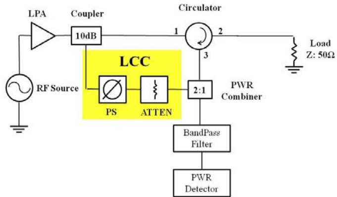
Figure 27. Basic LCC testing schematic.
