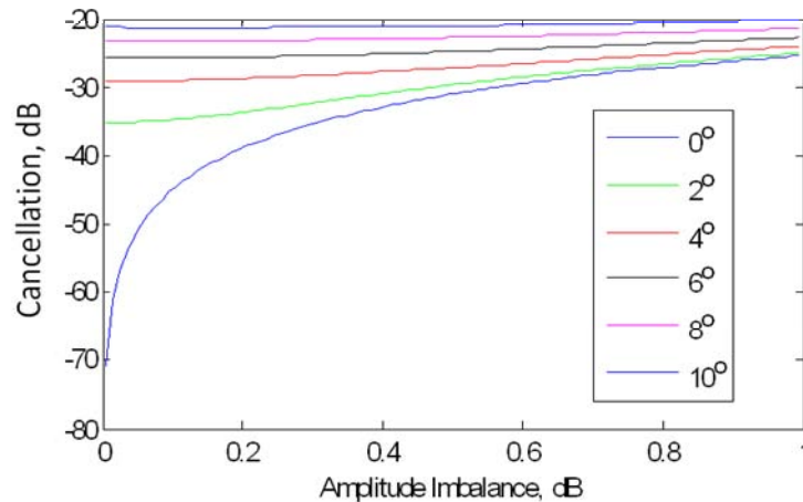
Figure 14. Effect of phase and amplitude imbalance (From [11]).
