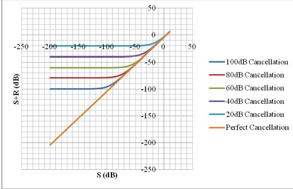
Figure 23. Cancellation level testing.
