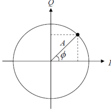
Figure 37. The in-phase (I) and quadrature (Q) plane (From [12]).
