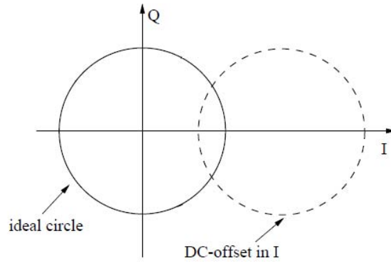
Figure 44. DC offset error (From [12]).
