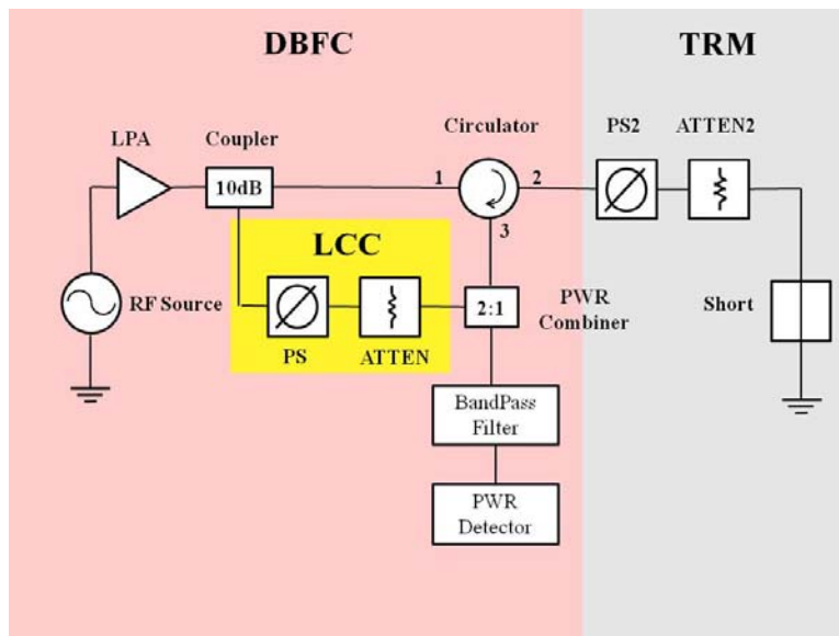
Figure 34. Modified TRM and DBFC test configuration.
