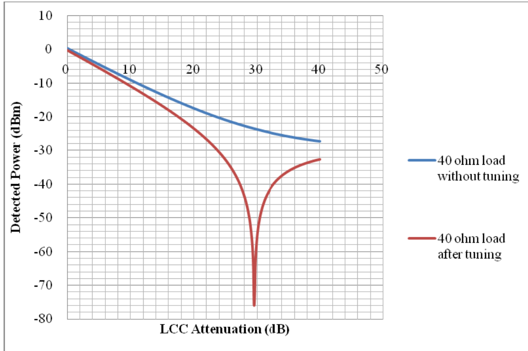
Figure 18. Mismatch tuning simulation result.
