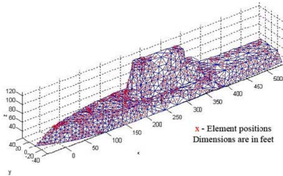
Figure 2. CAD model of Zumwalt-class sized ship with 1200 randomly distributed antenna elements (From [2]).
