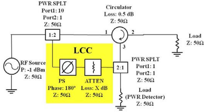
Figure 12. DBFC simulation configuration.
