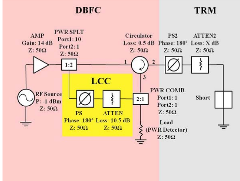
Figure 20. DBFC and TRM configuration.
