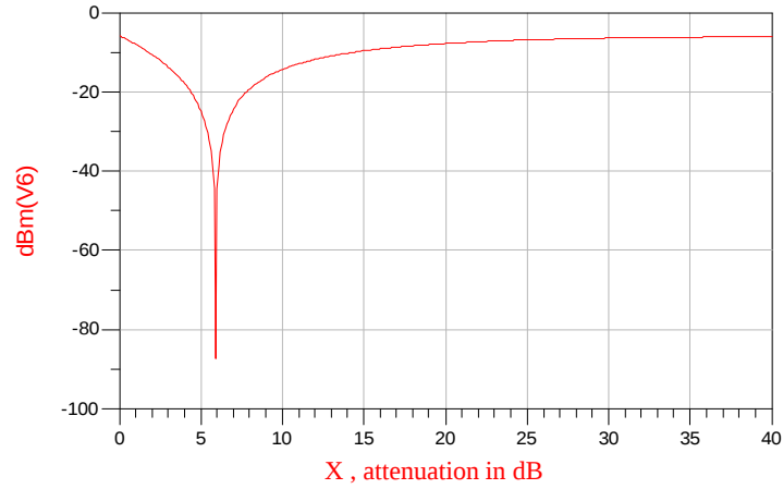
Figure 11. Example of a 40 dB sweep in attenuation.
