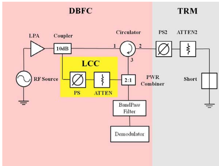
Figure 39. DBFC and TRM test diagram.
