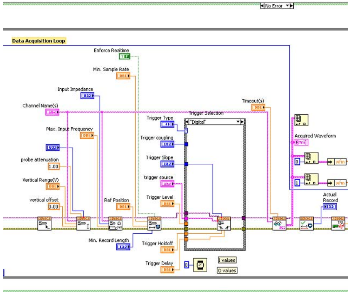
Figure 26. LabVIEW block diagram example.
