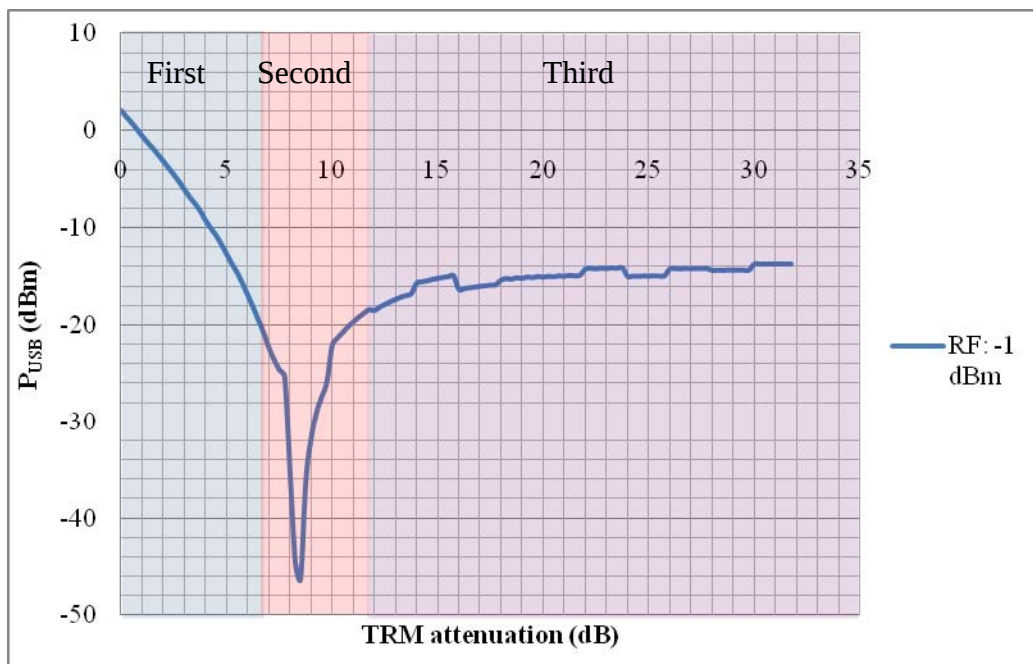
Figure 35. TRM and DBFC measurements.
