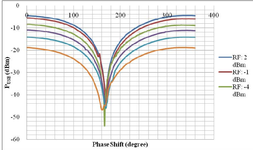
Figure 32. LCC measured result (with mechanical attenuator).
