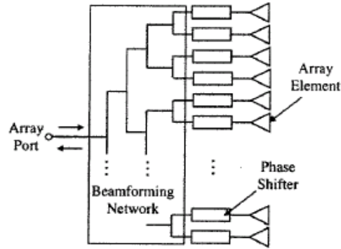
Figure 3. Analog BFN (From [3]).
