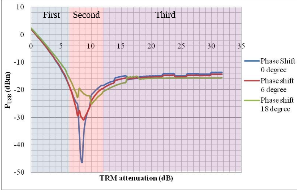
Figure 36. TRM phase mismatch measurements.
