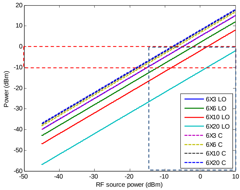
Figure 55. Coupler selection result (X = 6 dB).
