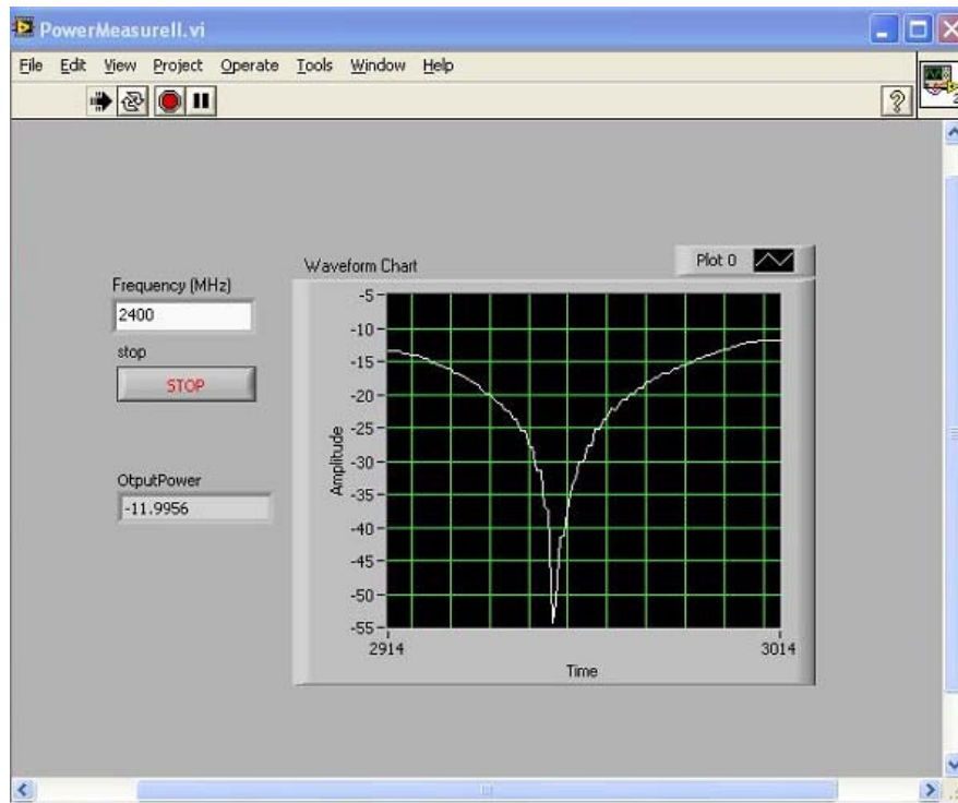
Figure 28. Power measurement front panel.
