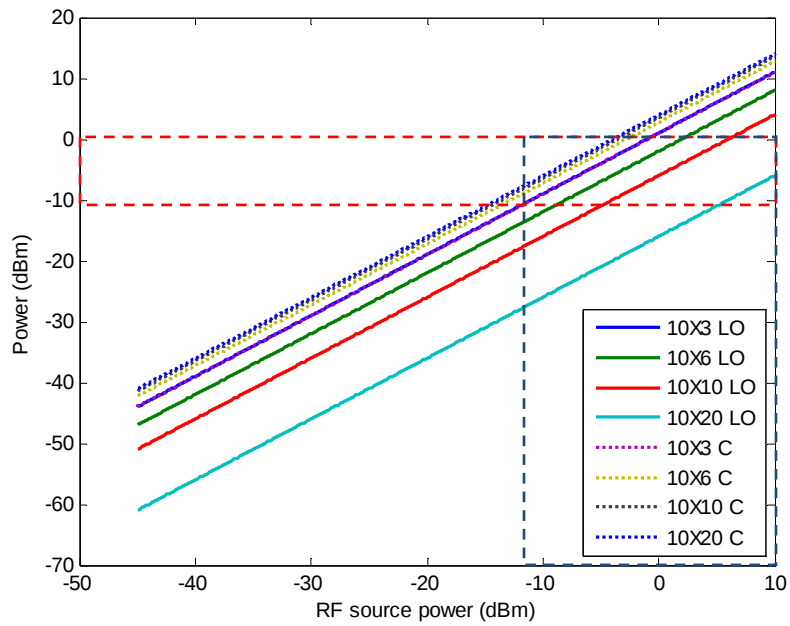
Figure 56. Coupler selection result (X = 10 dB).
