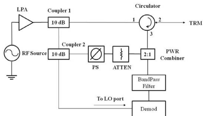
Figure 58. Finalized DBFC test configurations.
