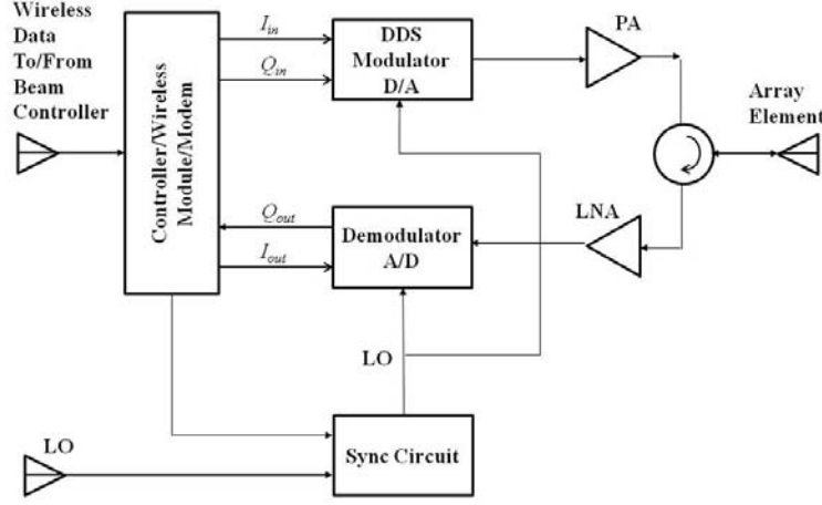
Figure 6. TRM block diagram (After [4]).
