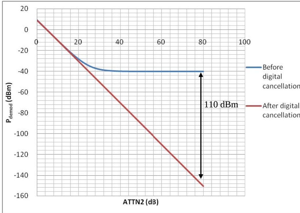
Figure 40. DBFC and TRM simulation results before and after digital correction.
