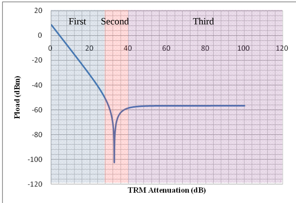
Figure 21. Power received at 50 Ω load.
