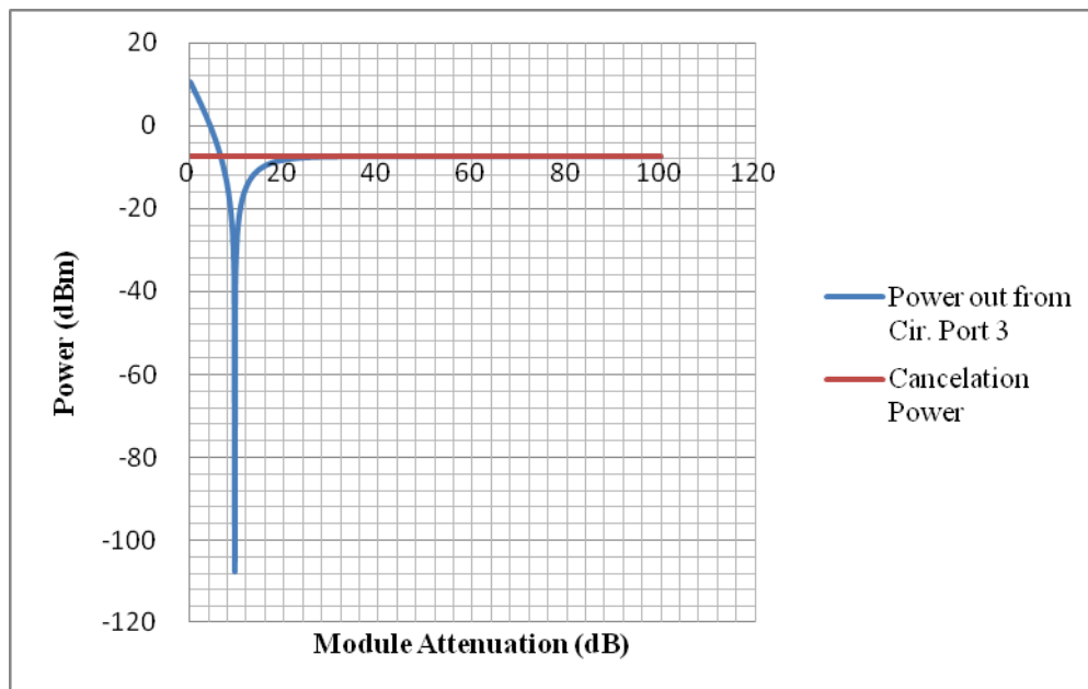
Figure 22. Power from LCC and circulator port 3.
