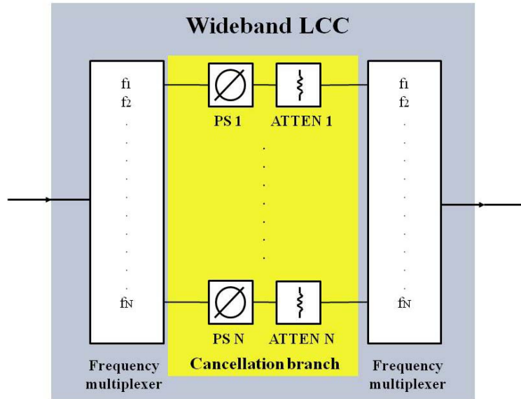
Figure 59. Wideband leakage cancellation circuit using N channels.
