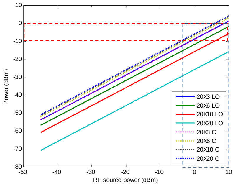
Figure 57. Coupler selection result (X = 20 dB).
