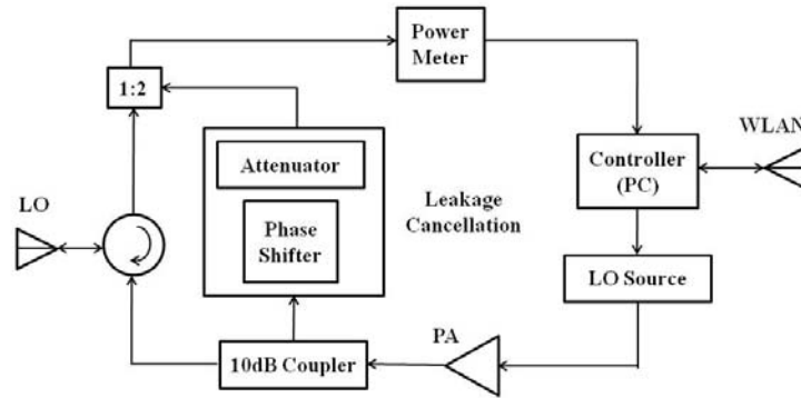
Figure 5. DBFC block diagram (From [4]).
