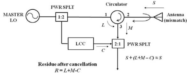
Figure 13. Operation of the LCC.
