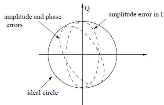
Figure 43. Phase and amplitude error (From [12]).
