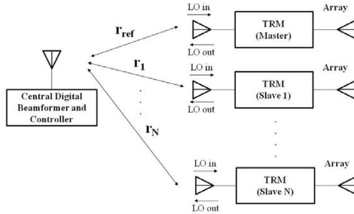
Figure 7. Sequential synchronization illustration.
