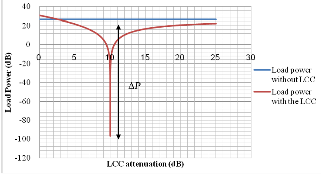
Figure 15. Example of \Delta P calculation.
