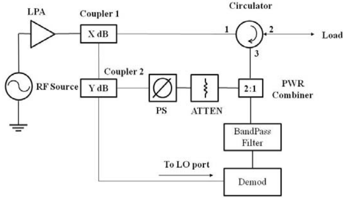
Figure 53. New DBFC test diagram.
