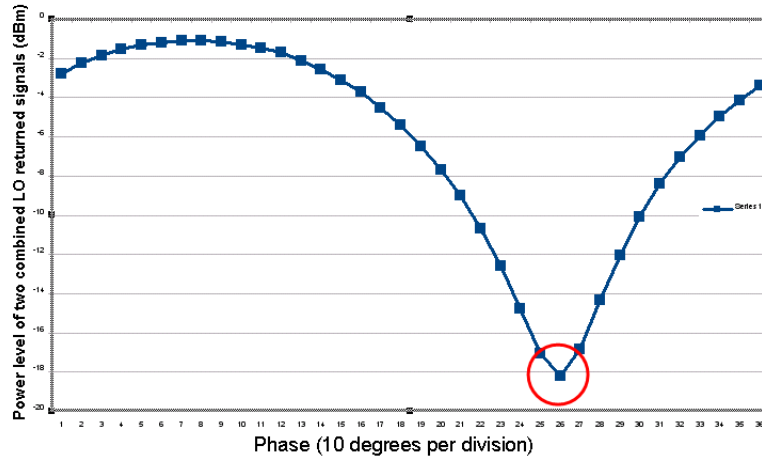
Figure 8. Demonstrated phase comparison algorithm (From [4]).
