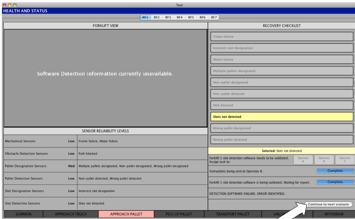
Figure 30: Recovery screen after correct confirmation, Traditional Checklist.
