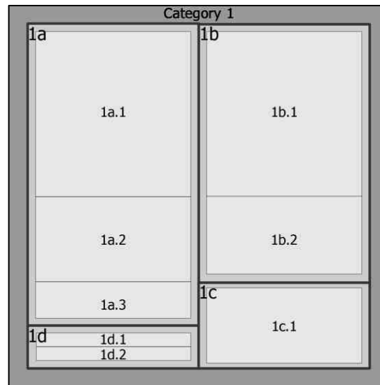
Figure 6: Treemap visualization.
