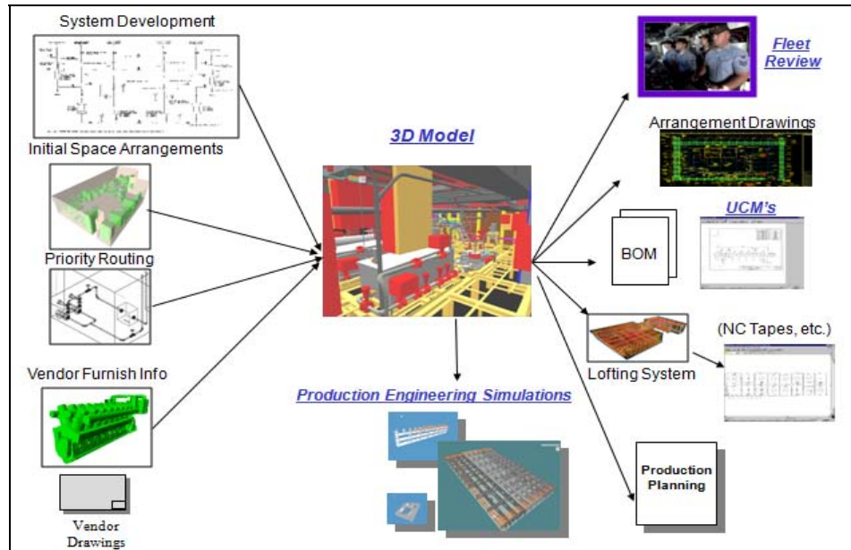
Figure 20. Information Can Be Imbedded Directly into 3D Model (From Murphy, 1997)
