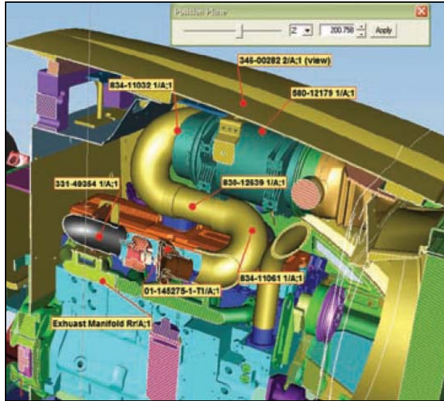
Figure 9. Enhanced 3D Product Model
