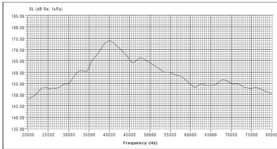
Figure 24. Source level (untuned) at 0° measured by Teledyne Benthos. From [5]
