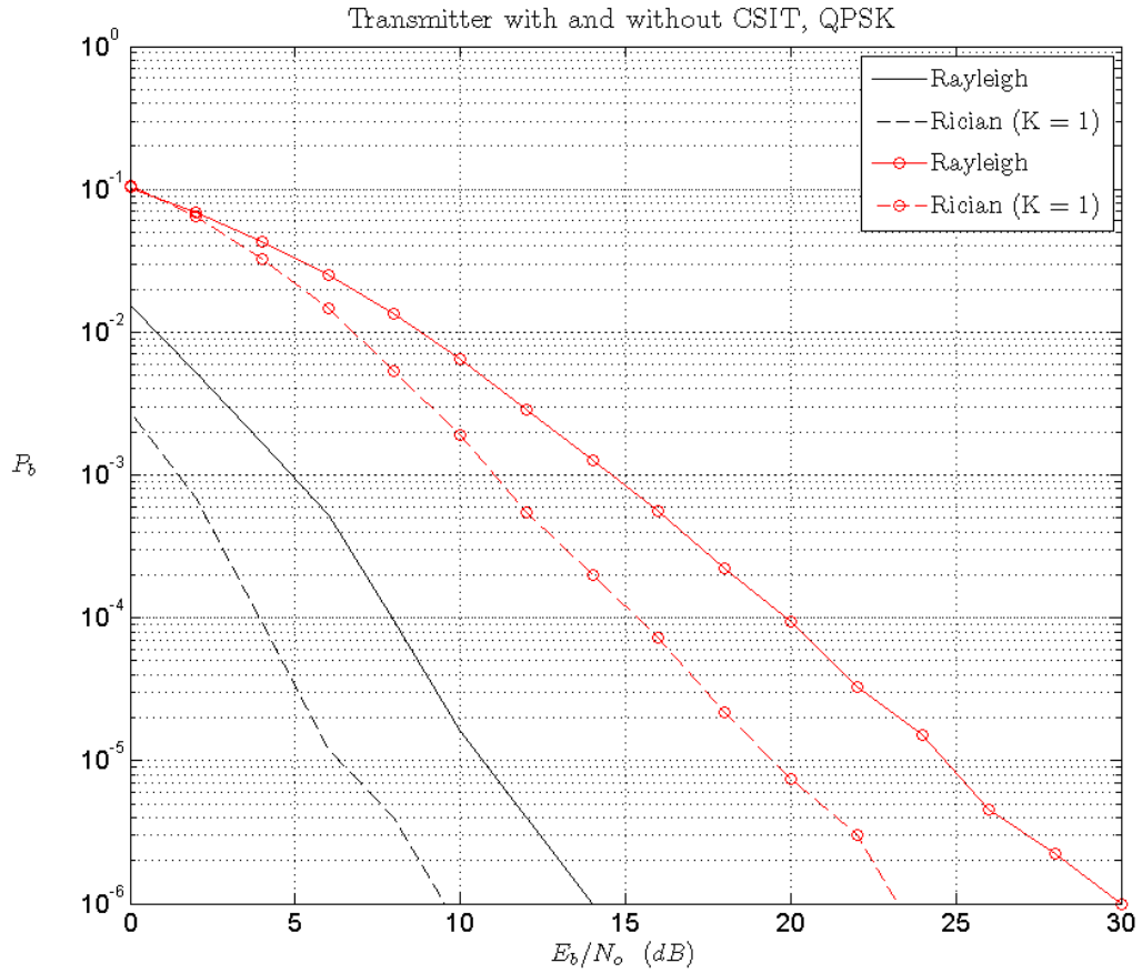
Figure 37. Simulated BER performance of a transmitter with and without CSIT for a 2x2 MIMO system in various channels using QPSK modulation.
