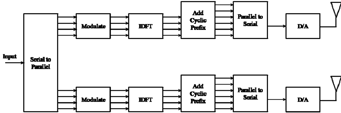
Figure 5. OFDM-MIMO Transmission Block Diagram (After [2]).
