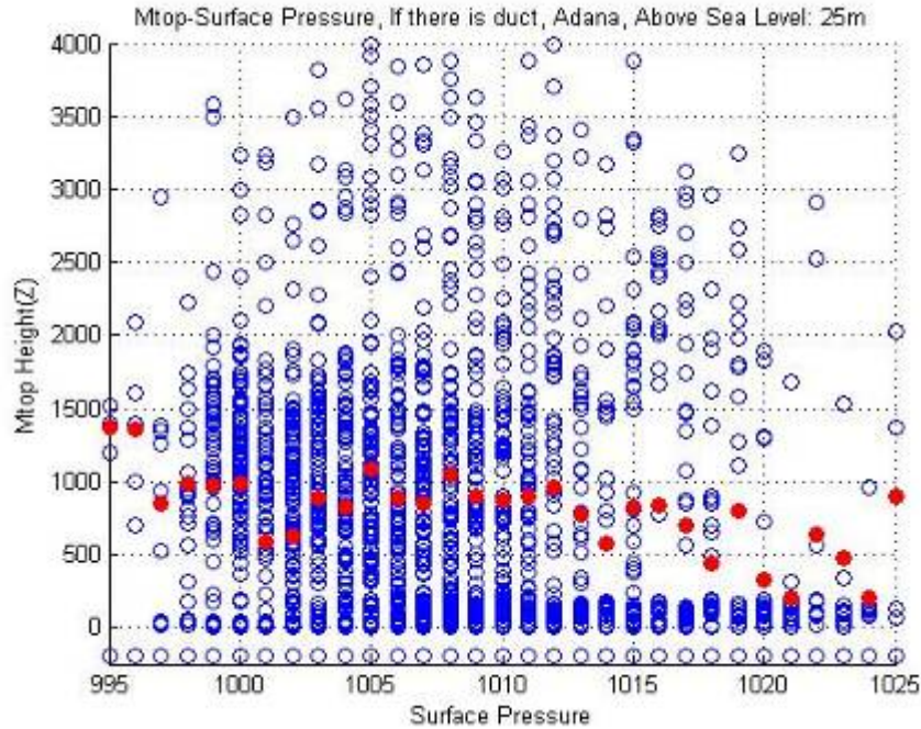
Figure 20. Height (m) and Surface Pressure (millibar) Correlation for Adana (if a Duct Presents)
