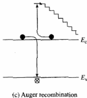
Figure 9. Recombination Methods (From [9]).
