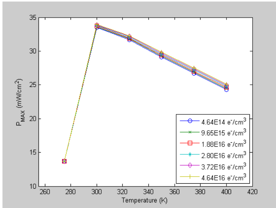
Figure 53. GaAs Emitter Doping - P_{\text{MAX}} versus Temperature.
