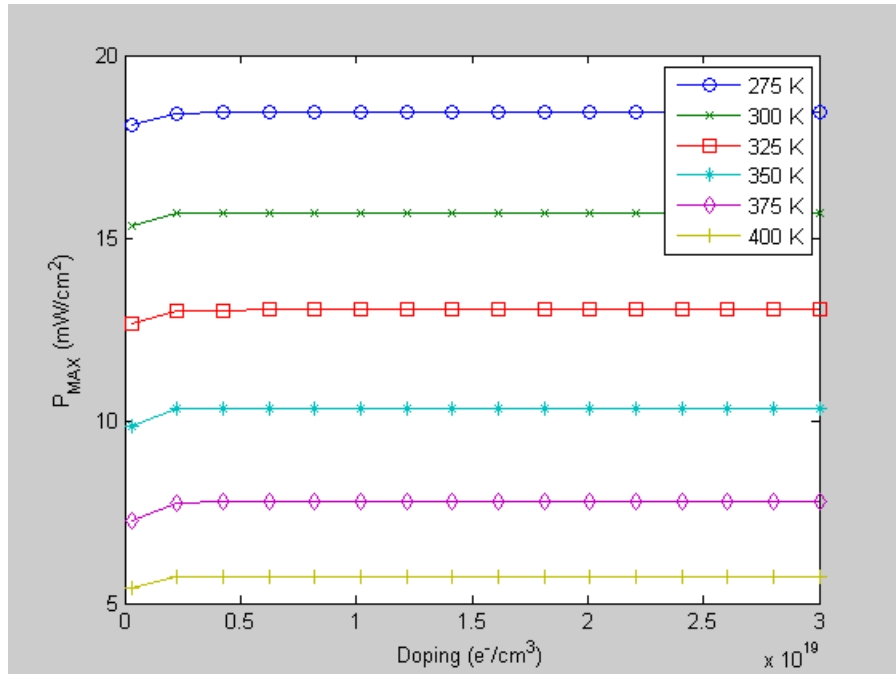
Figure 44. Ge - P_{\text{MAX}} versus Emitter Doping (275-400 K).
