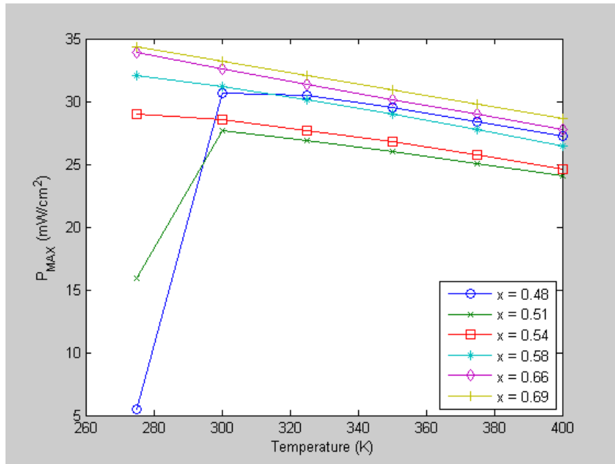
Figure 67. \text{In}_{1-x}\text{Ga}_x\text{P} - P_{\text{MAX}} versus Temperature.
