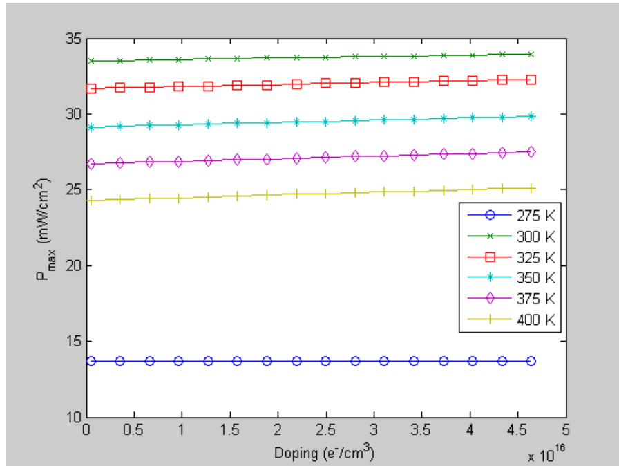
Figure 52. GaAs - P_{\text{MAX}} versus Emitter Doping (275-400 K).
