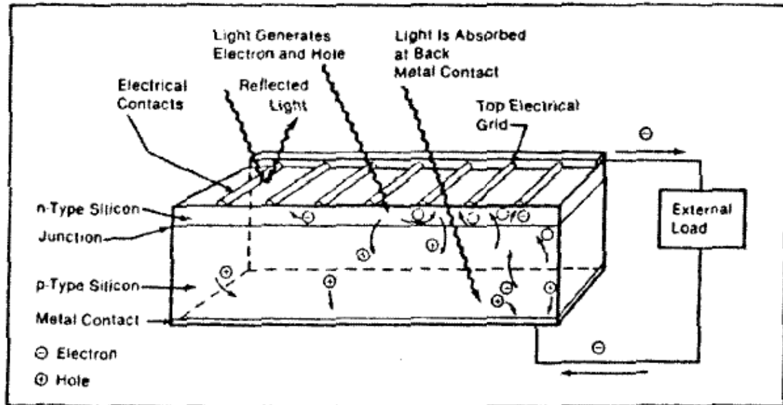
Figure 15. Solar Cell Operation (From [10]).
