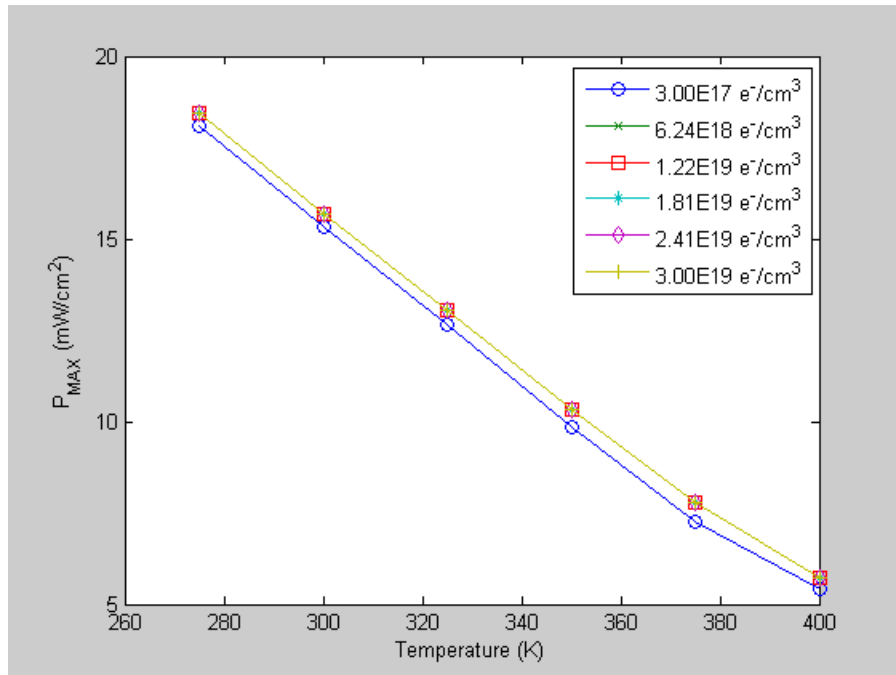
Figure 45. Ge Emitter Doping - P_{\text{MAX}} versus Temperature.
