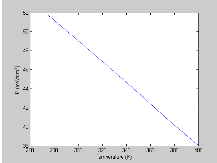
Figure 29. P_{MAX} Versus Temperature.
