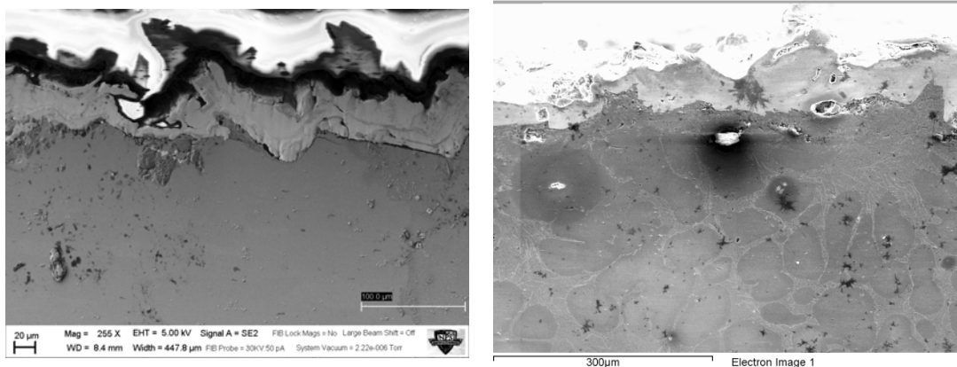
Figure 34. Scanning electron image of: Unprocessed material before (left) and after (right) flat tool FSP. FSP material consistently shows reduced porosity, less cracking at the interface, and a more even Titanium distribution along the surface.
