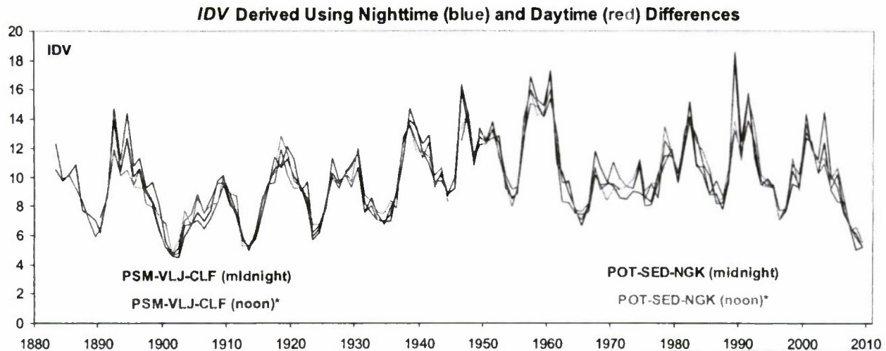
Figure 6. Raw IDV derived using nighttime hourly data (blue) and daytime hourly data (red) for the French stations PSM-VLJ-CLF and the German stations POT-SED-NGK. The daytime values are \sim 30\% larger than the nighttime value because of day-to-day (non-solar) variations of the regular solar variations, S_R , and have been scaled to the same average as the nighttime values for easier comparison.
