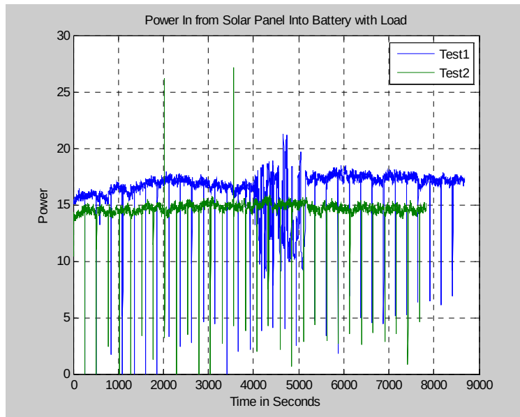
Figure 50. Power Input to Load w/SP Test.
