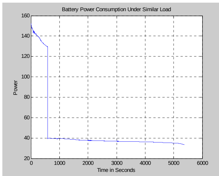
Figure 47. Power Consumption 100% to 55% Similar Load.
