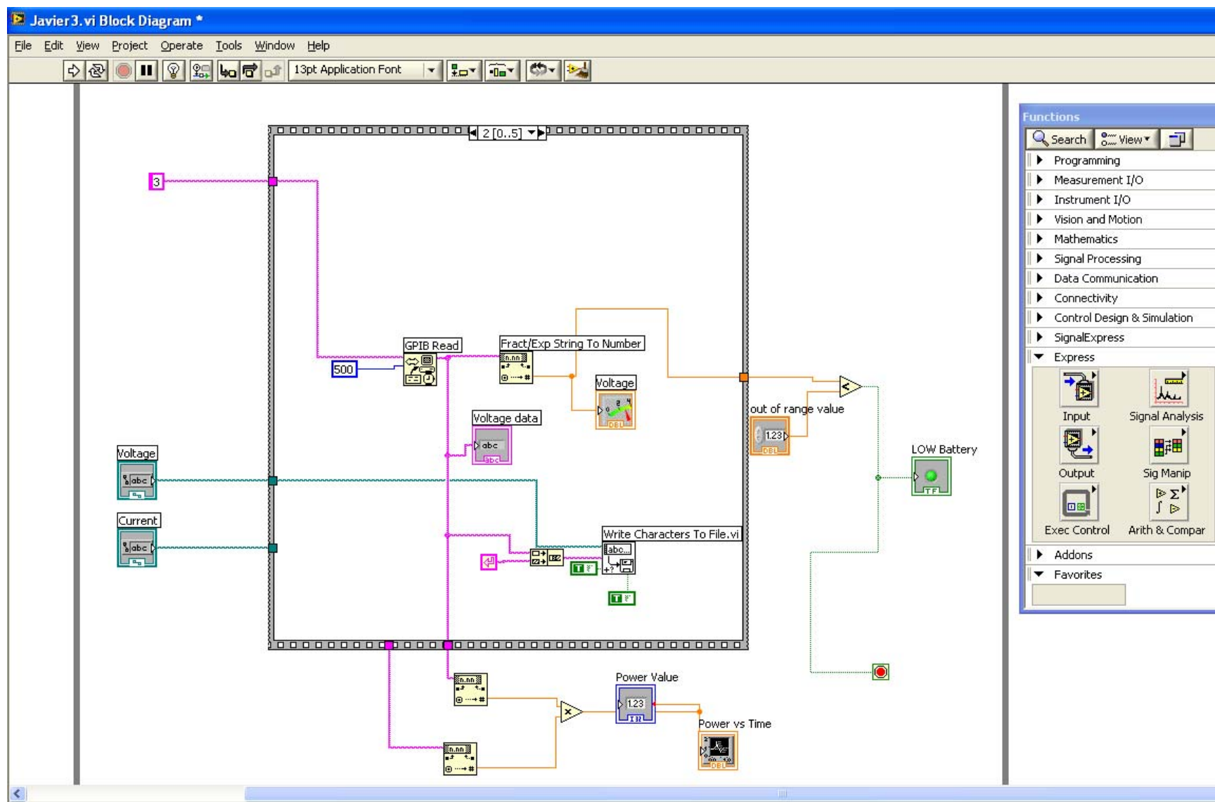
Figure 41. LABVIEW Block Diagram.
