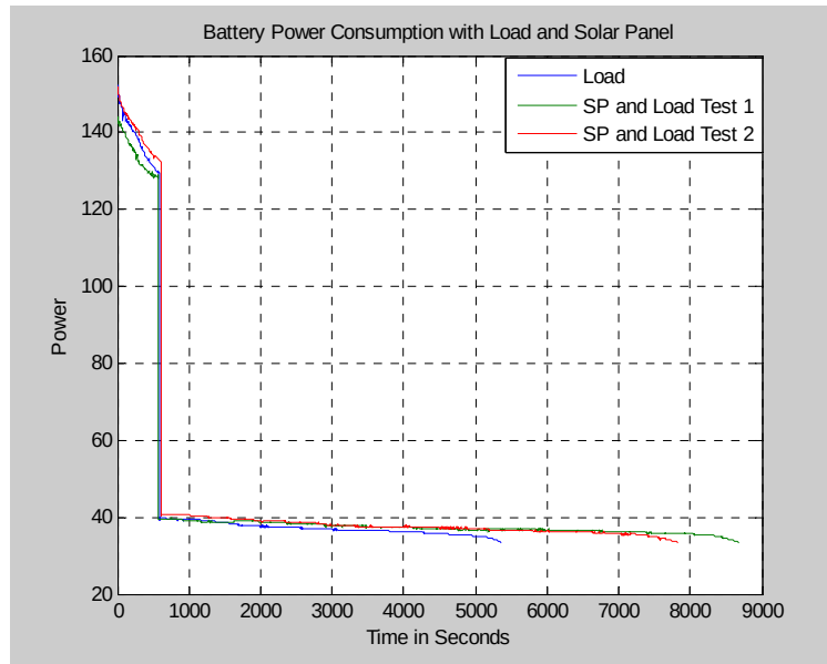
Figure 51. Power Consumption Load w/ Solar Panel.
