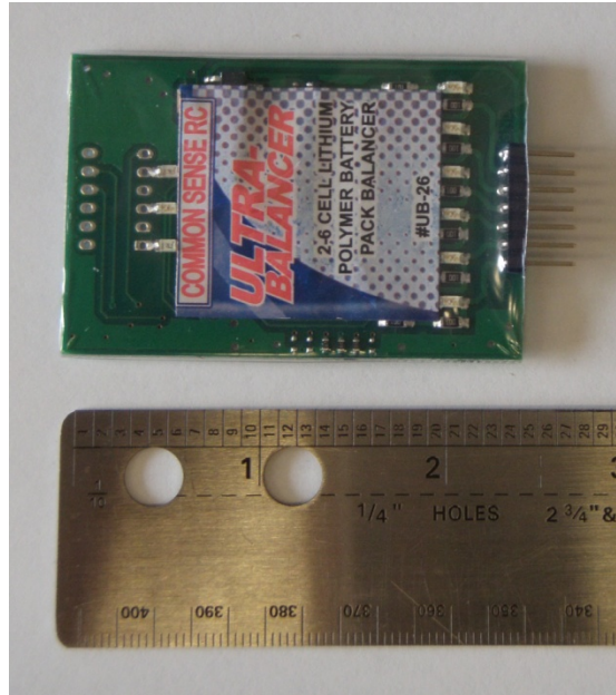
Figure 37. Ultra-Balancer Charger.
