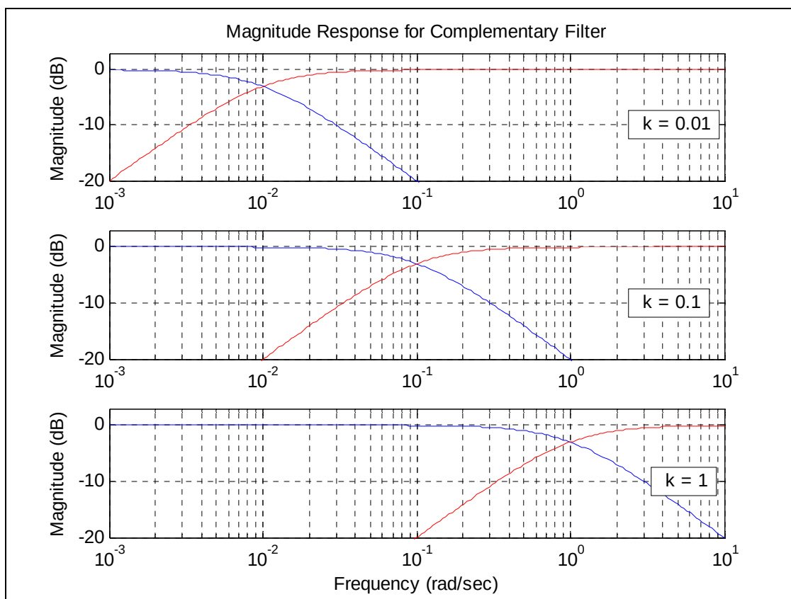
Figure 27. Magnitude response of static branch (blue) and dynamic branch (red).
