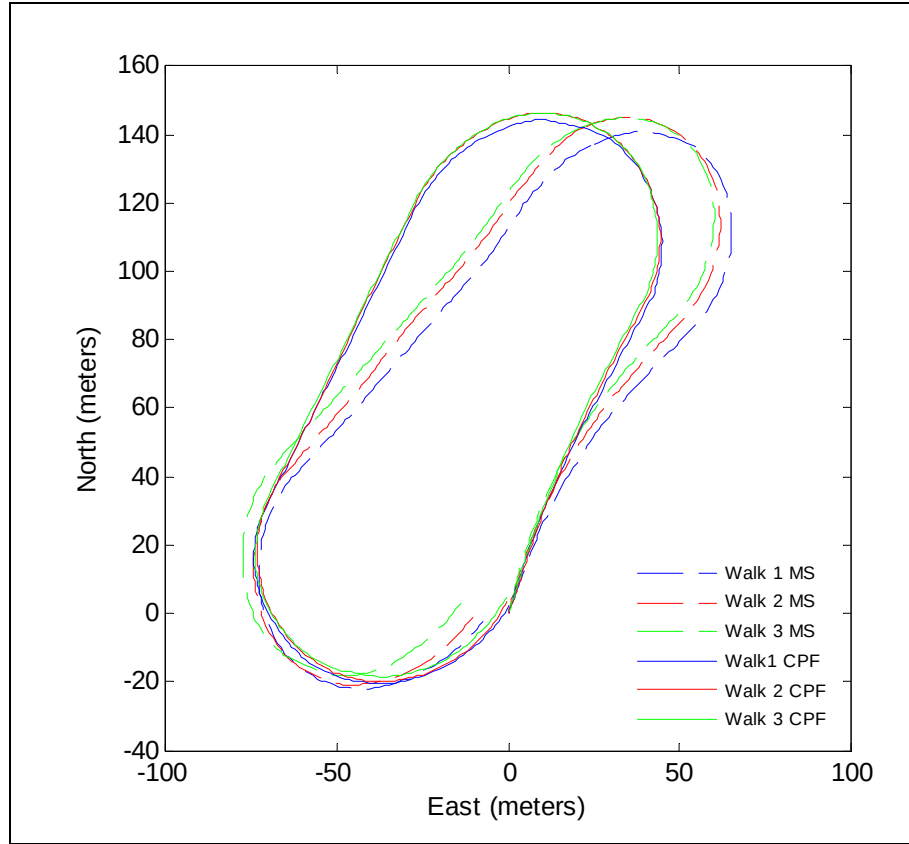
Figure 90. Comparison of position track using adaptive-gain complementary filter (solid) and proprietary algorithm (dashed).
