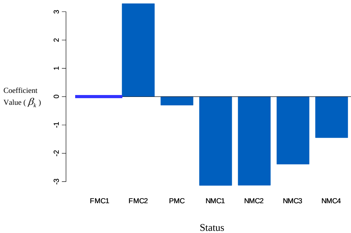
Figure 5. Bar chart of the Status.Prior coefficients from the logistic regression used in Model 14. Larger positive values indicate greater likelihood of availability.
