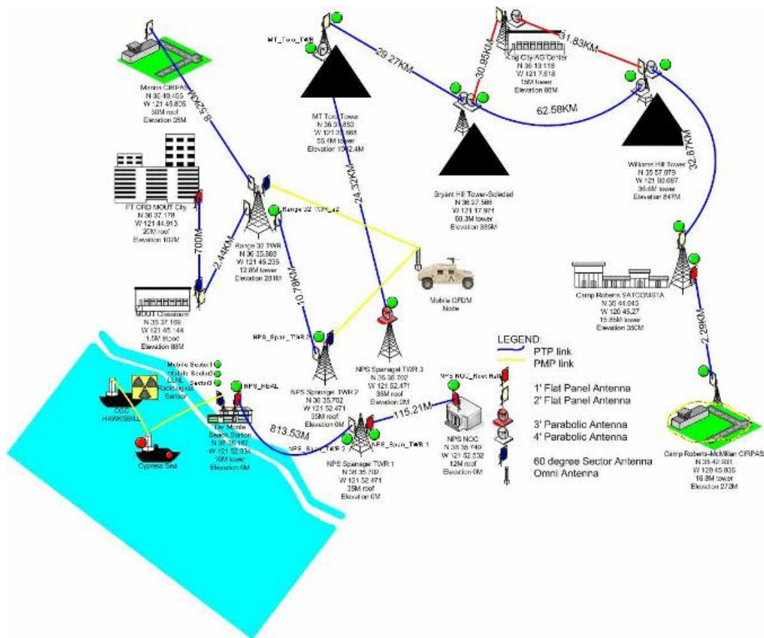
Figure 8. OFDM backbone of NPS Tactical Network Topology test bed (From CENETIX site)
