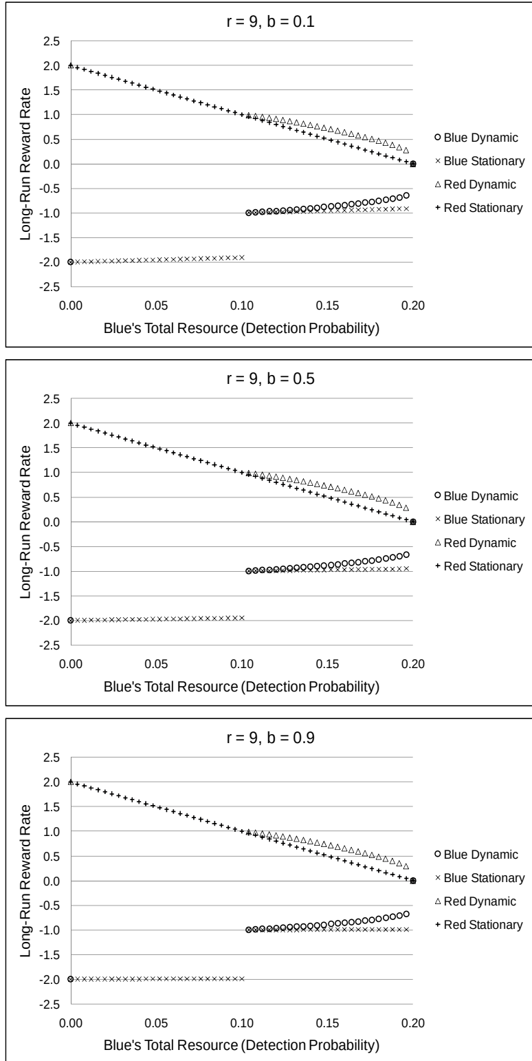
Figure 13. Comparison between dynamic allocation and stationary allocation with r = 9, b = 0.1, 0.5, 0.9
