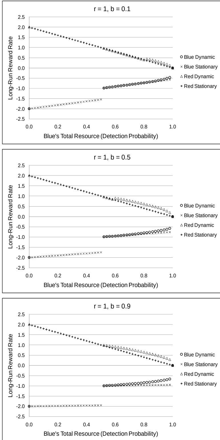
Figure 12. Comparison between dynamic allocation and stationary allocation with r = 1 , b = 0.1, 0.5, 0.9
