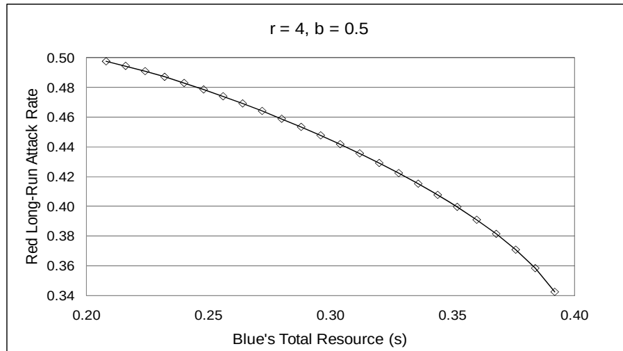
Figure 10. Red long-run attack rate in dynamic allocation, compared with 0.5 in the case of stationary allocation.
