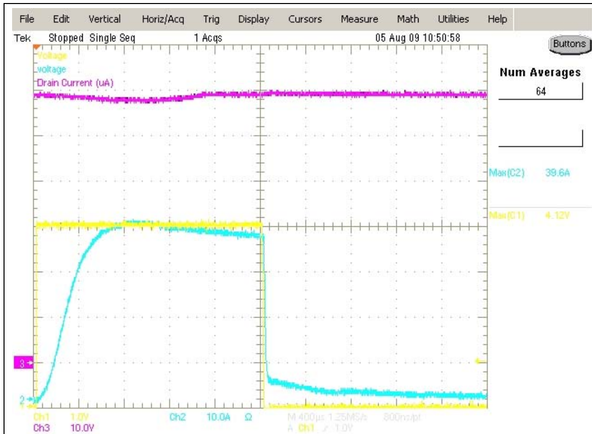
Figure 2. A good example of a current pulse.
