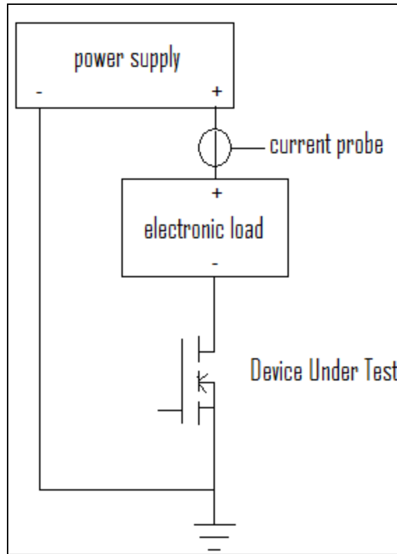
Figure 1. Circuit with supply and electronic load; DUT was not used.
