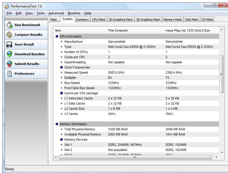
Figure VI-1: PerformanceTest 7.0 Screenshot
