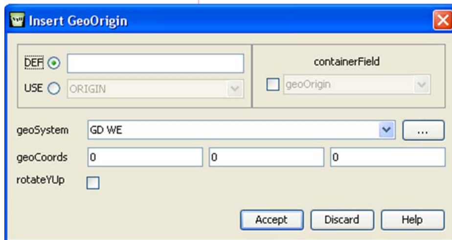
Figure 43. GeoOrigin Editing Panel in X3D Edit
