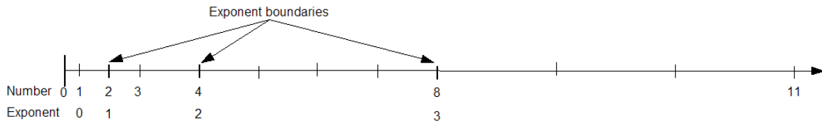
Figure 15. Floating Point Density (From Thorne, 2007)
