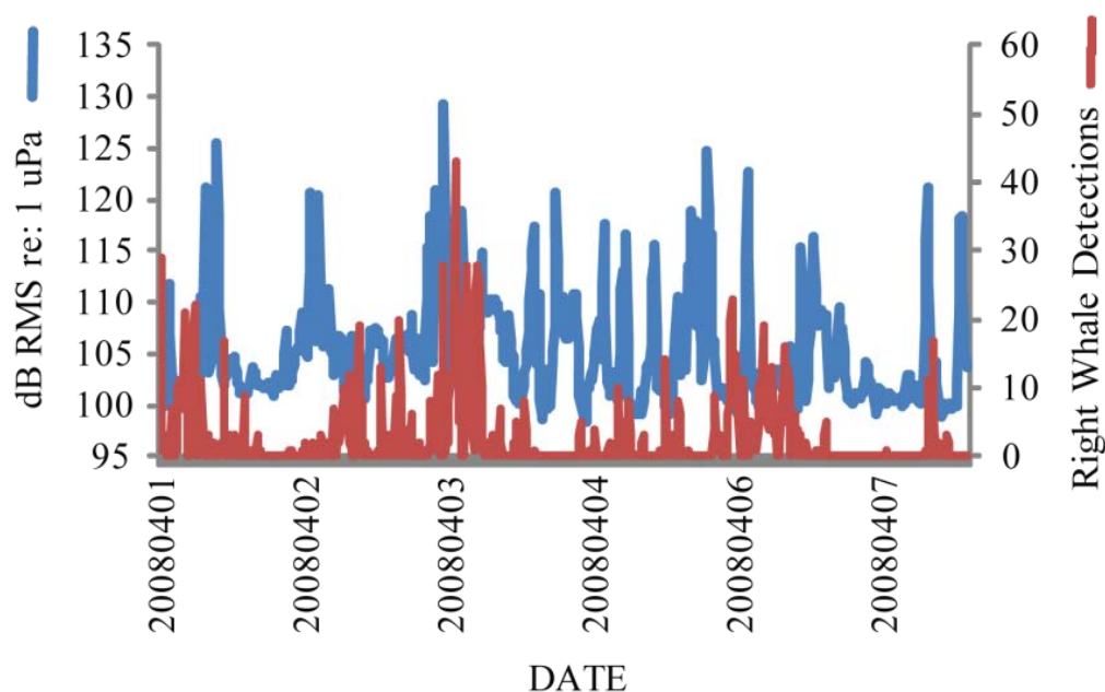
Figure 8. Received sound levels (blue, 30-400Hz dB re 1 \mu Pa) and numbers of detected right whale calls (red) for 15-minute time bins recorded on a single MARU in the array (Figure 2) on 1-7 April 2008.
