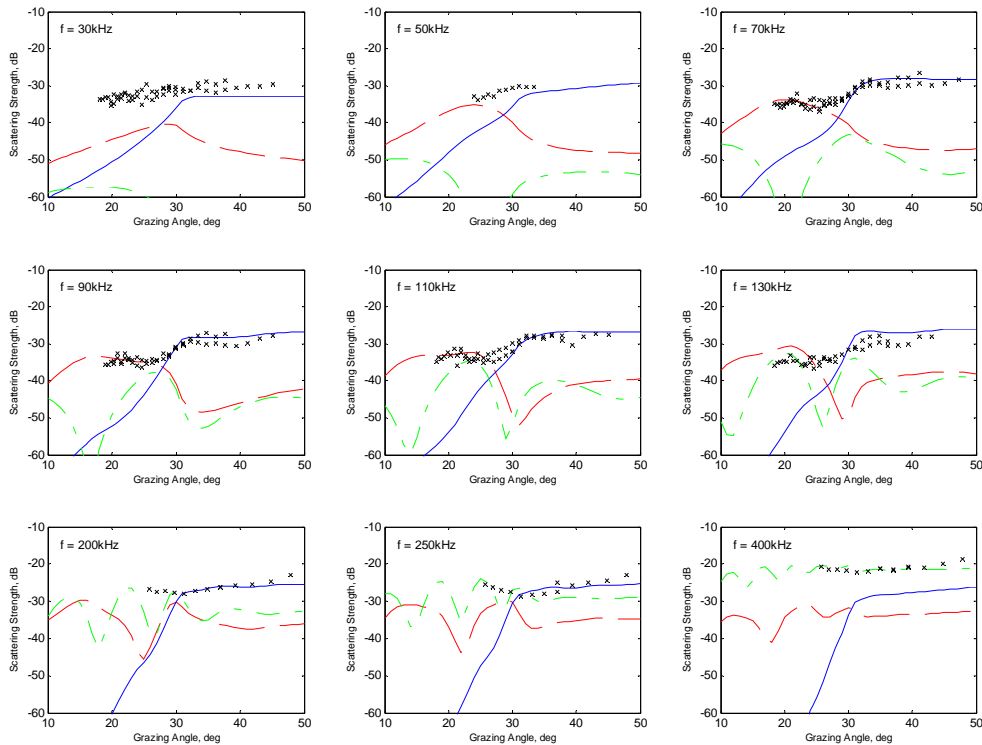
Fig. 4. Model/data comparisons: theoretical angular dependences of the bottom backscattering strength for the three types of inclusions, shown at different frequencies, 30 to 400 kHz, versus data measured at SAX04 by K. Williams [4].
