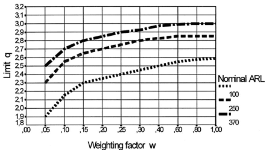
Figure 14. Determining the limit q of the EWMA chart after selection of w and the nominal ARL from Neubauer 1997
