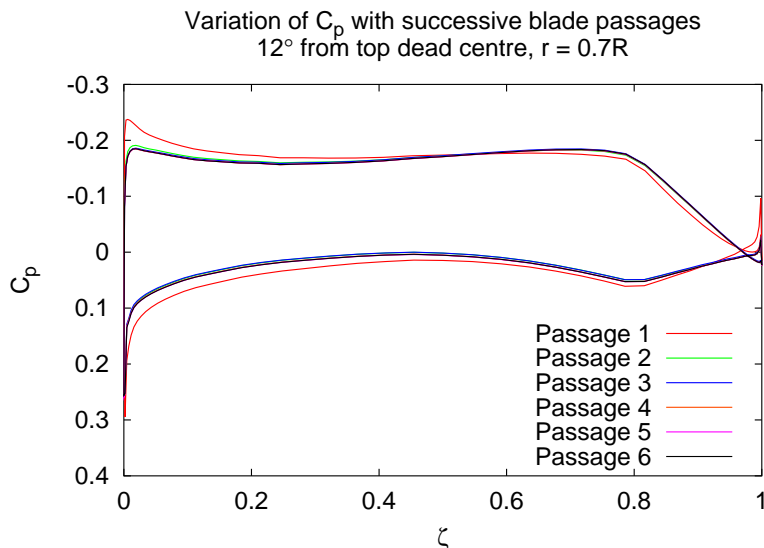
Figure 8: The variation of C_p with successive blade passages. Each curve represents C_p at r = 0.7R on a single blade as it passes the location 12° past top dead centre in the direction of rotation.
