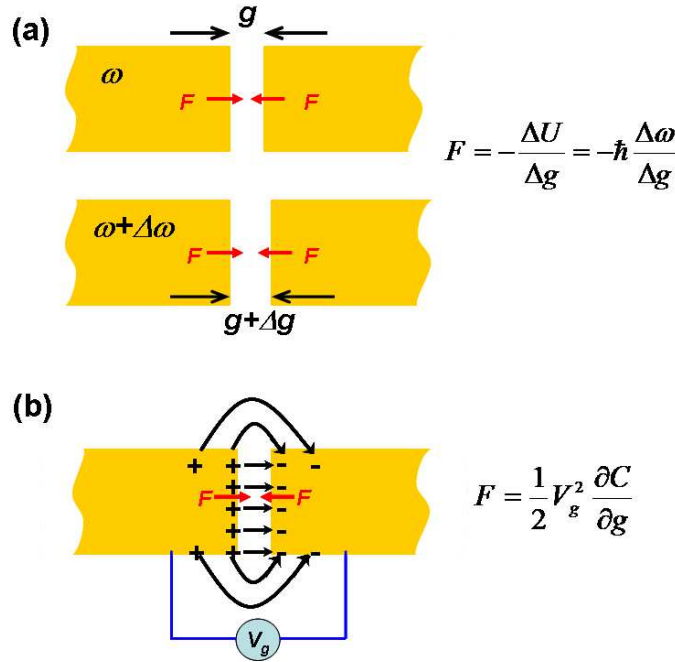
Fig. 1. (a) Schematic of an optical dipole antenna, whose resonance frequency depends on the gap width. The optical force is given as a differentiation of the energy (resonance frequency) with respect to the gap width. (b) In the electro-static picture, the force is a Coulomb force resulting from the opposite charge accumulation on the two electrodes
