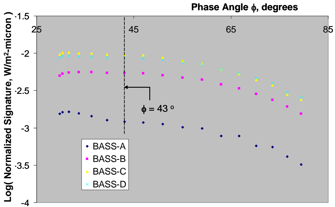
Figure 1b: Range Normalized Signature for Satellite-B (Observation ID: 86-080916-1401)
