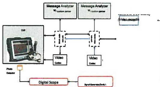
Figure 6: Video Latency
