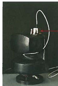
Rate Gyro positioned to Measure panning of PTZ
