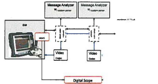
Figure 5: Latency Measure C2 --> Actuator on PTZ
