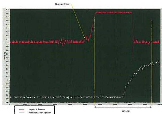
Figure 9: Latency Measure
