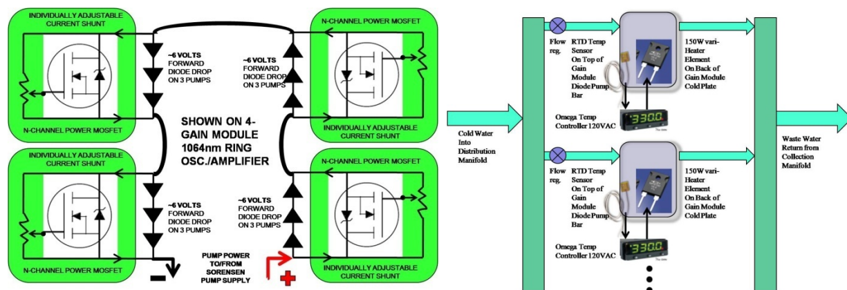
Fig. 3 A diagram of the current and temperature tuning systems for FASOR-X. These control systems are some of the major upgrades in FASOR-X over the SOR FASOR and will result in a more robust system that is easier to use.
