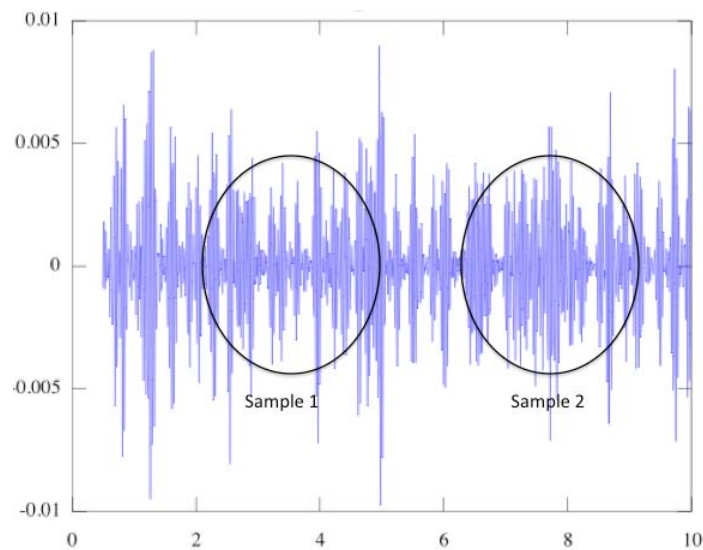
Figure 5. Kurtosis Example
