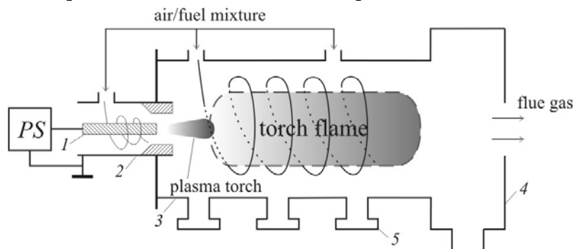
Fig. 1. Schematic arrangement of a system for plasma assisted combustion. 1 – inner electrode of a nonsteady-state plasmatron; 2 – grounded outer electrode of plasmatron; 3 – combustion chamber; 4 – unit for flue gas diagnostics; 5 – auxiliary windows.
