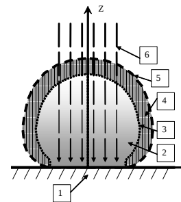
Fig.1 The outline of laser plume structure. 1 – metallic target; 2 – The erosion vapor area; 4 – The area of shock – compressed gas.
