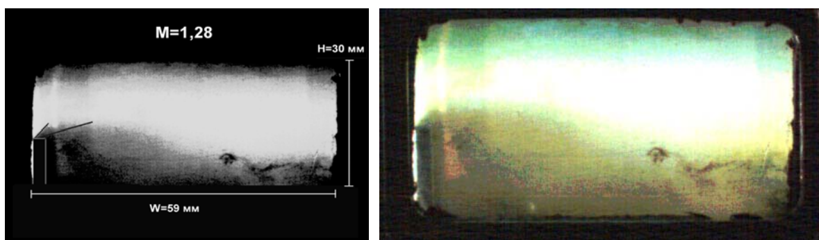
Figure 2. Plasma flow of the rectangular wall. Exposition time - 5 ms. a) Picture after the graphic working b) original picture
